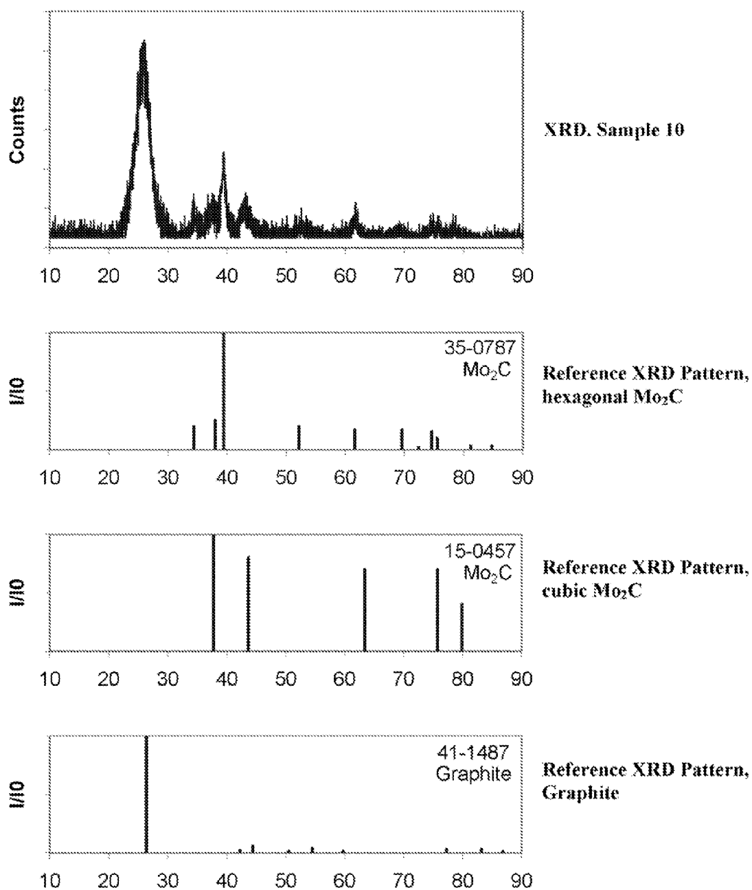
FIG. 3A XRD and HRTEM of CARBIDE NANOPARTICLES SUPPORTED ON CARBON NANOTUBES
