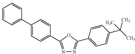
Oxadiazole-containing compound
