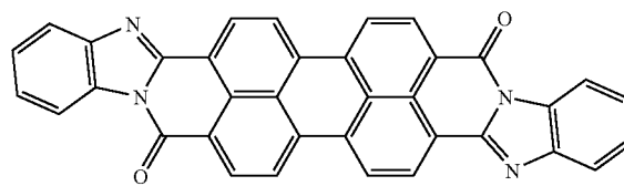
Perylene-based compound
