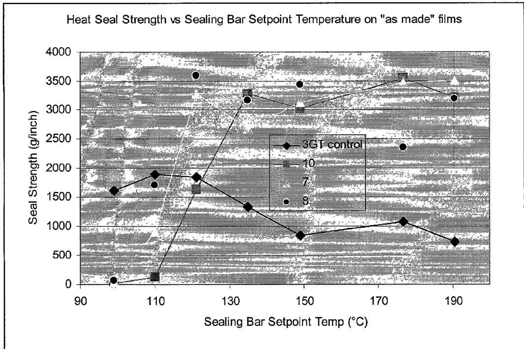
FIG. 4 Heat Seal Strength on "As Made" Films
