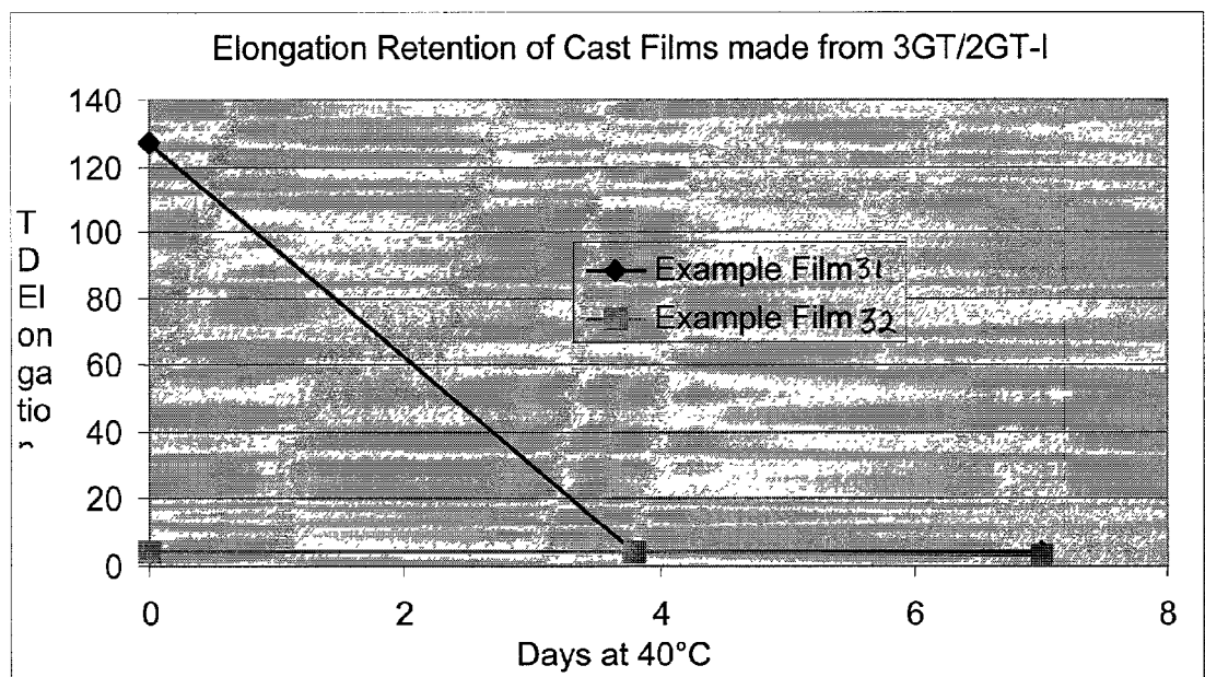
Fig. 30 Average TD Elongation to break for example films 31 and 32 before and after the conditioning at 40°C.
