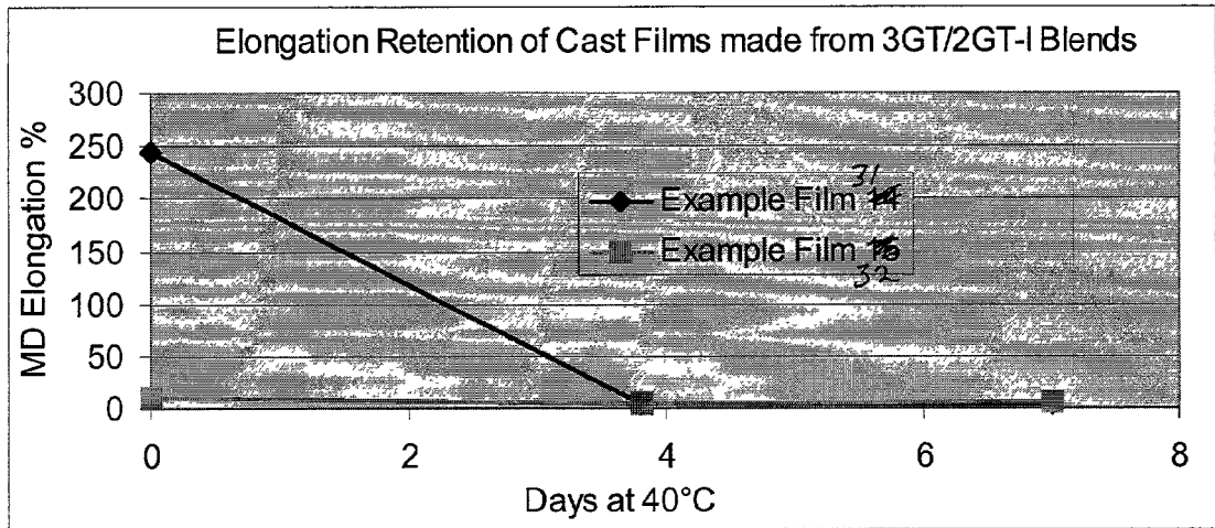
Fig. 29 Average MD Elongation to break for example films 31 and 32 before and after the conditioning at 40°C.
