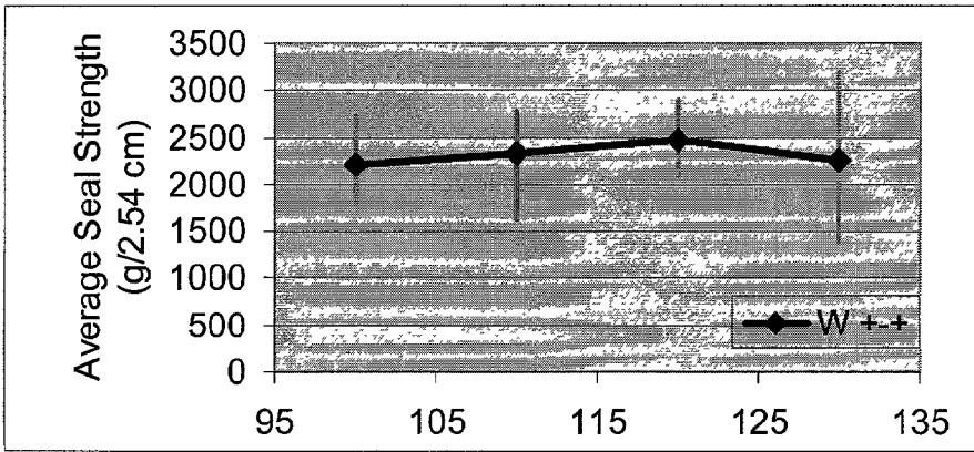
FIG. 24 – Average Seal Strength (Showing Max and Minimum Value) for Example Film X
