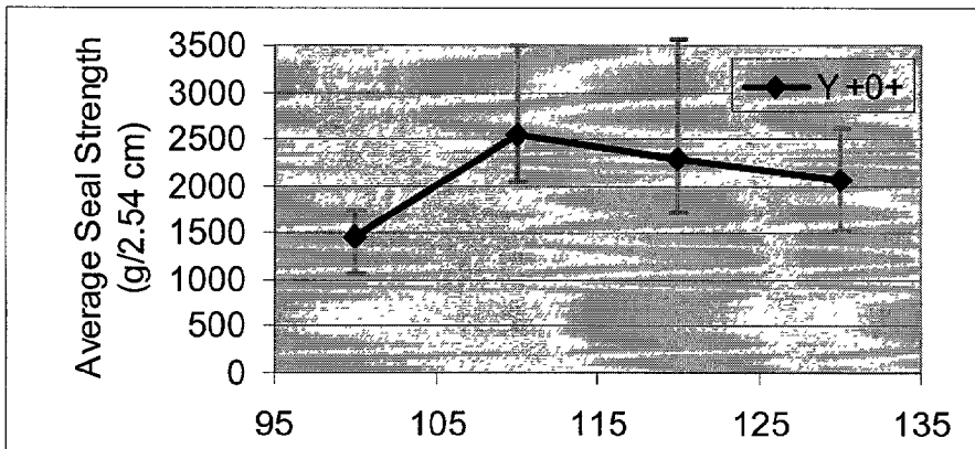
FIG. 25 – Average Seal Strength (Showing Max and Minimum Value) for Example Film Y
