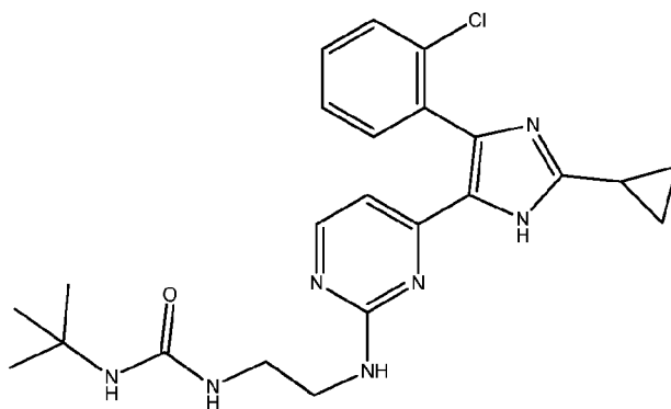
Compound 27
