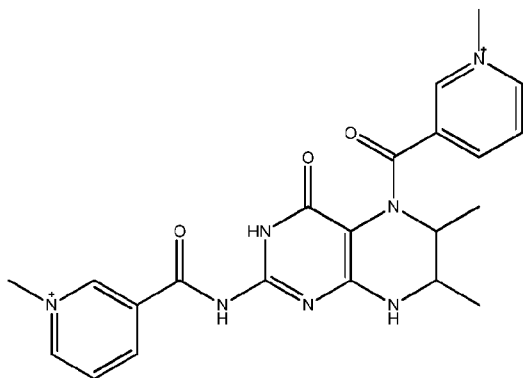
Compound 7
