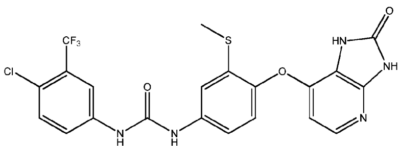
Compound 37
