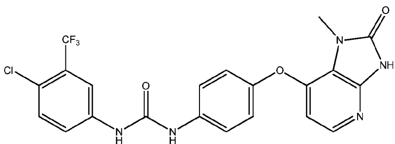
Compound 35
