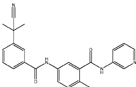
Compound 20
