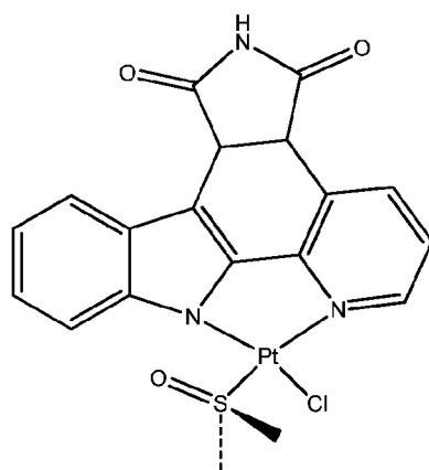
Compound 14
