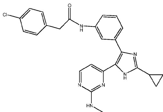
Compound 31
