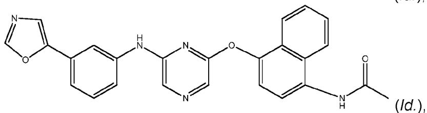
Compound 25
