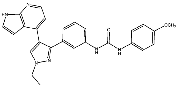
Compound 33
