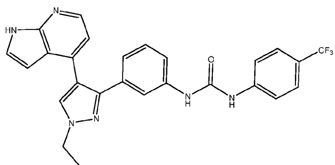
Compound 32
