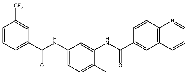
Compound 18
