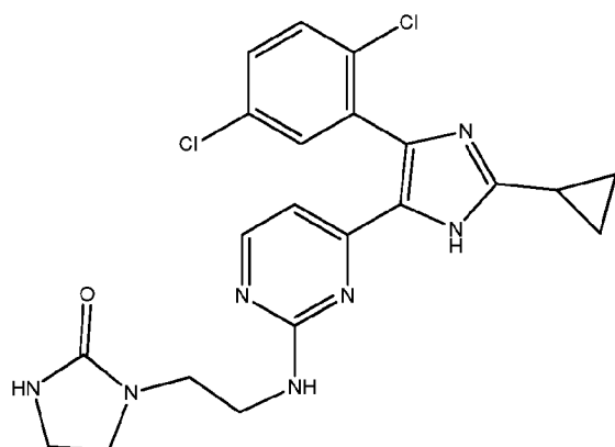
Compound 28
