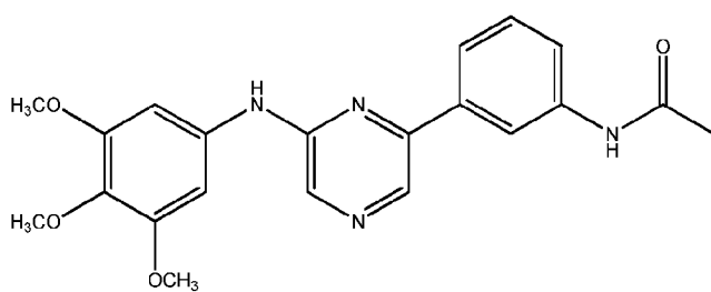
Compound 21
