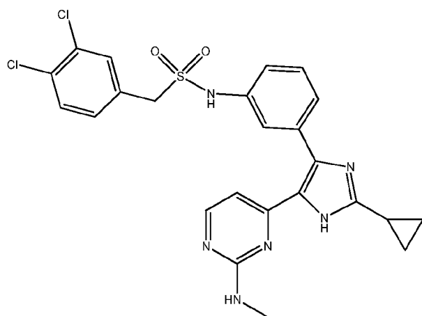
Compound 30
