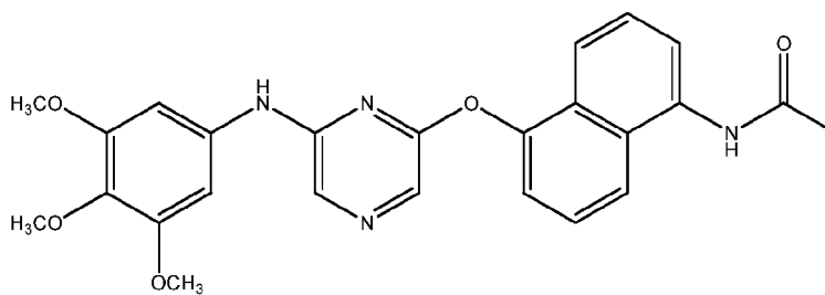
Compound 24
