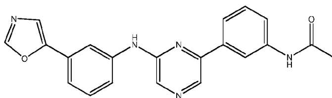
Compound 22
