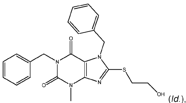
Compound 10
