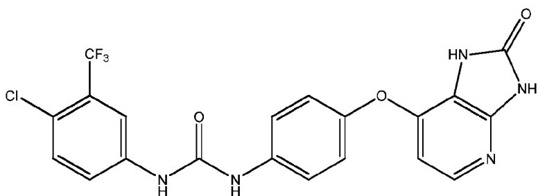
Compound 34
