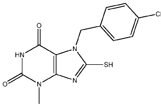
Compound 9
