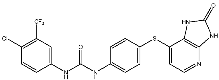
Compound 36
