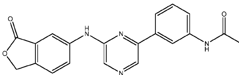
Compound 23
