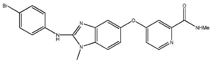
Compound 16
