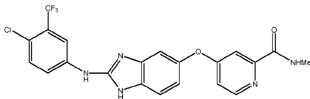
Compound 15
