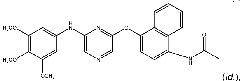
Compound 26
