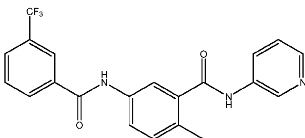
Compound 19
