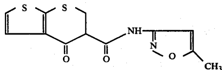
5,6-Dihydro-N-(5-methyl-3-isoxazolyl)-4-oxo-4H-thieno[2,3-b]-thiopyran-5-carboxamide
