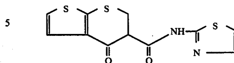
5,6-Dihydro-4-oxo-N-(2-thiazolyl)-4H-thieno[2,3-b]-thiopyran-5-carboxamide
