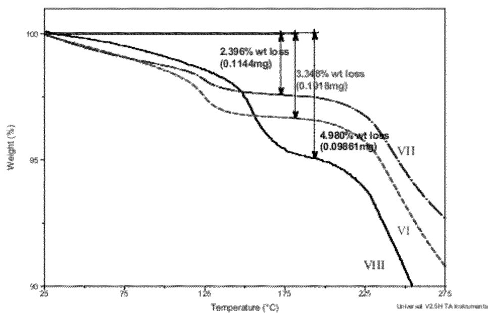
Figure 4. TGA curves of solids from solvents \text{CH}_2\text{Cl}_2 (Form VI), Hexane (Form VII), and acetonitrile (Form VIII).
