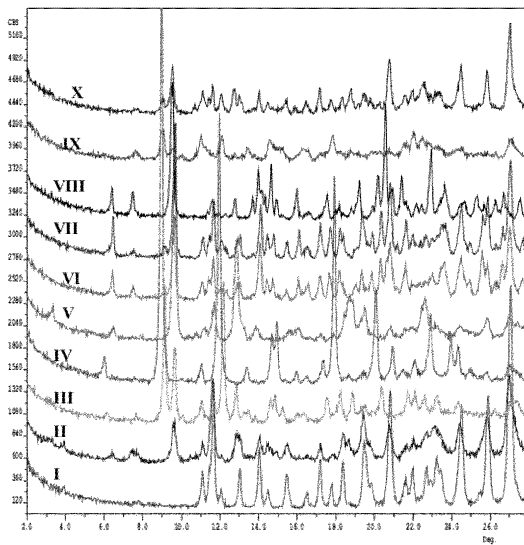
Figure 3. Powder X-ray Diffraction patterns of the ten unique polymorphs of Compound I.
