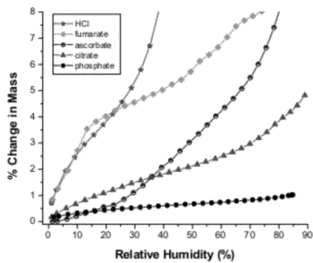
Figure 1. Moisture sorption data for salts of Compound I.
