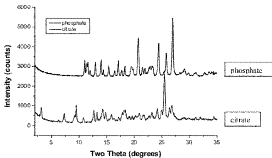
Figure 2. Powder X-ray Diffraction patterns for Compound I citrate and Compound I phosphate.
