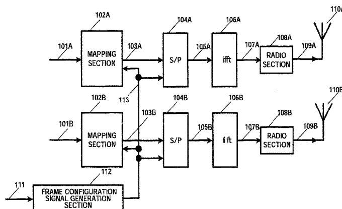
100 MIMO-OFDM TRANSMISSION APPARATUS
