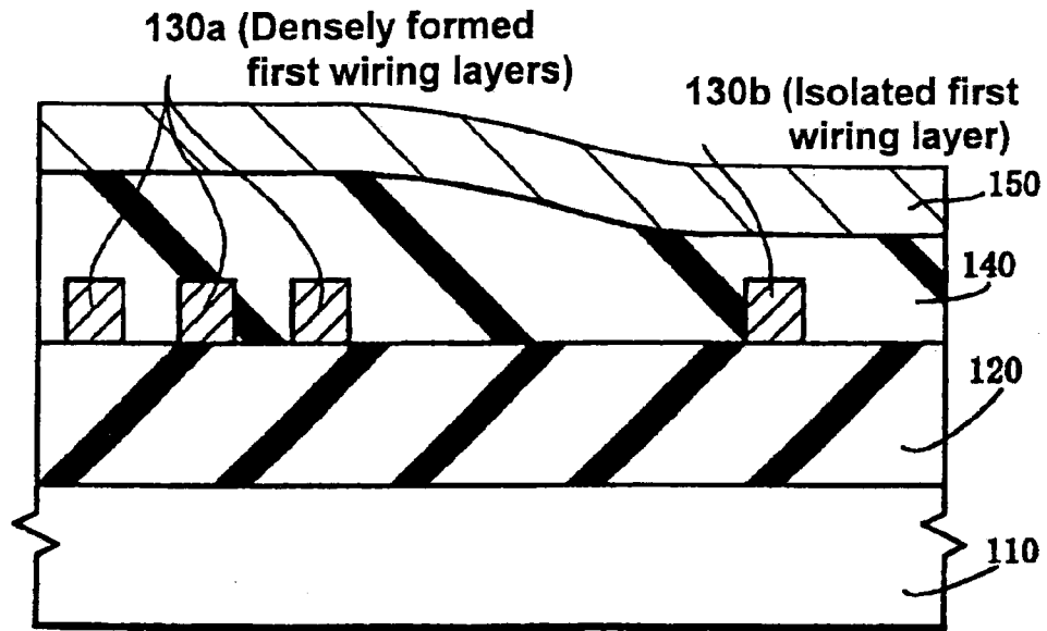
Fig. 18 (Prior Art)
