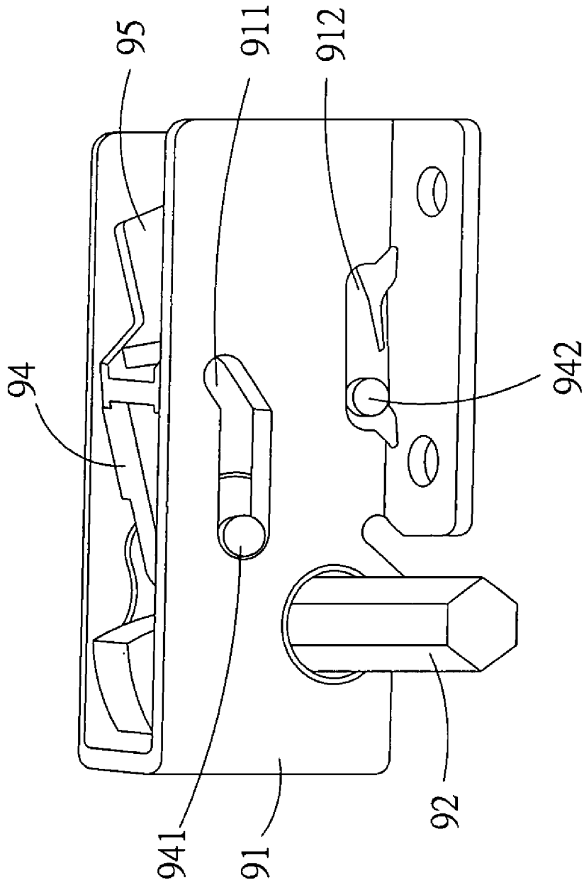
FIG 9 (PRIOR ART)
