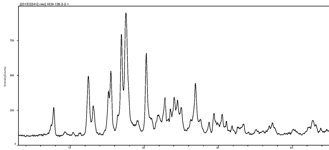
FIG. 8 XRPD Form III
