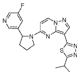
Chemical Compound 13
