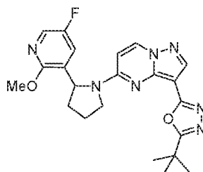
Chemical Compound 28
