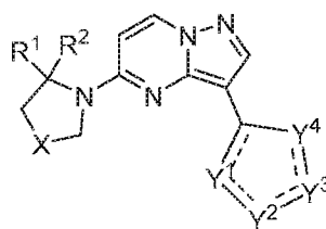
Formula III
