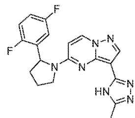
Chemical Compound 32
