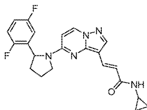
Chemical Compound 43
