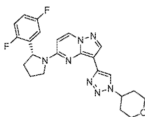
Chemical Compound 36
