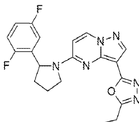
Chemical Compound 3
