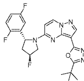
Chemical Compound 26
