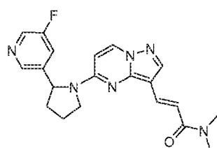
Chemical Compound 40
