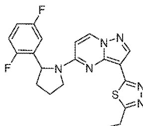
Chemical Compound 4
