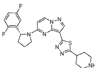
Chemical Compound 24
