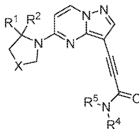
Formula IV
