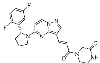
Chemical Compound 51
