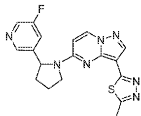
Chemical Compound 11
