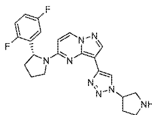
Chemical Compound 35
