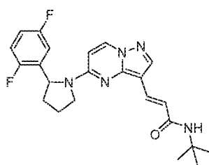
Chemical Compound 44
