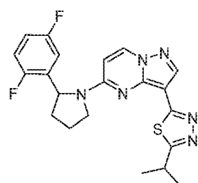
Chemical Compound 6
