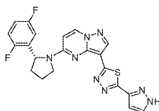
Chemical Compound 20
