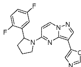
Chemical Compound 29
