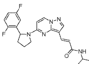
Chemical Compound 42
