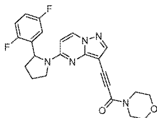
Chemical Compound 61
