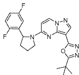
Chemical Compound 9
