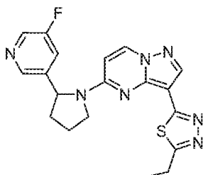
Chemical Compound 12
