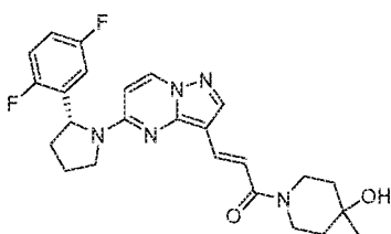
Chemical Compound 58
