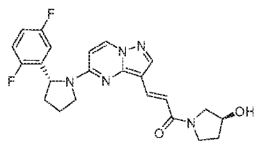
Chemical Compound 60
