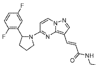
Chemical Compound 41
