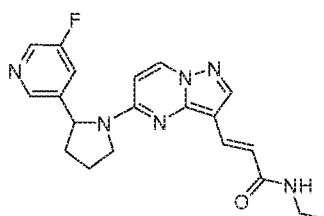
Chemical Compound 37
