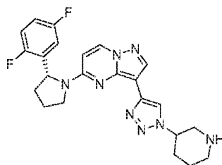
Chemical Compound 34
