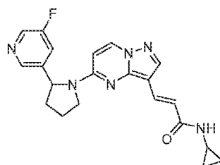
Chemical Compound 39
