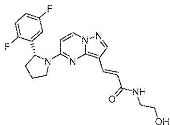
Chemical Compound 48
