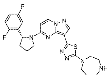
Chemical Compound 23
