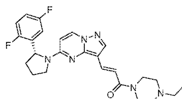
Chemical Compound 54
