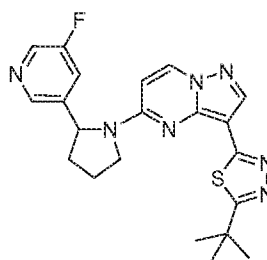
Chemical Compound 15
