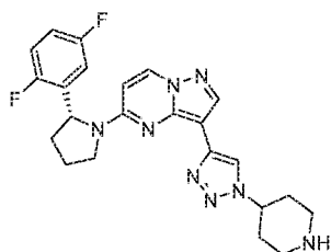
Chemical Compound 33
