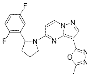
Chemical Compound 1
