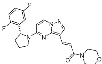
Chemical Compound 49
