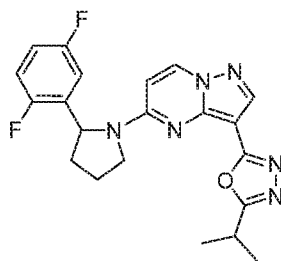
Chemical Compound 5
