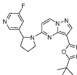
Chemical Compound 16
