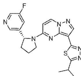
Chemical Compound 17
