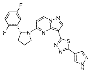
Chemical Compound 19
