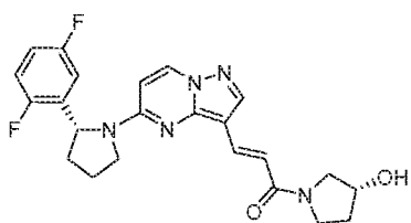
Chemical Compound 59
