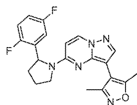
Chemical Compound 31
