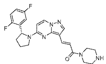
Chemical Compound 50
