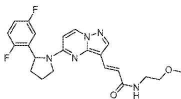
Chemical Compound 46
