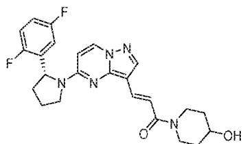
Chemical Compound 57
