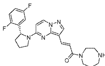
Chemical Compound 56
