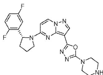
Chemical Compound 18
