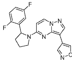
Chemical Compound 30
