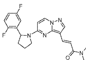
Chemical Compound 45
