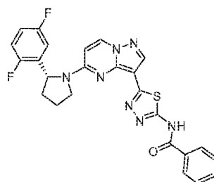
Chemical Compound 21
