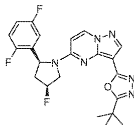
Chemical Compound 27
