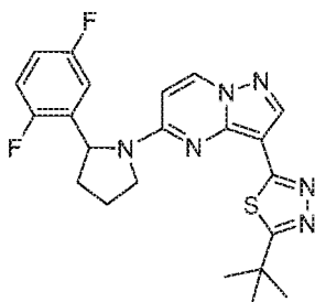
Chemical Compound 10
