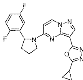
Chemical Compound 7
