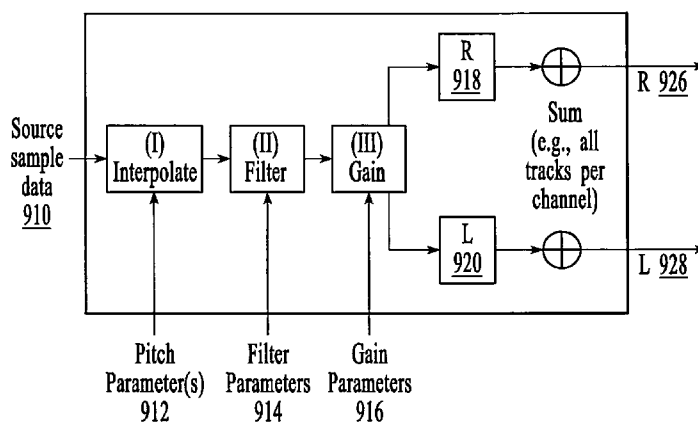
Exemplary Synthesis Structure
