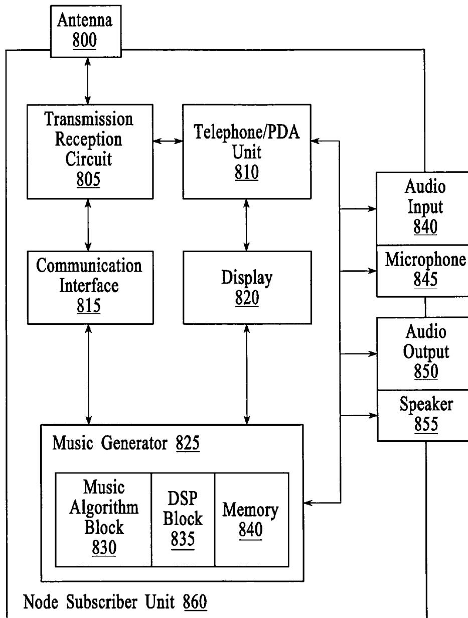
Node/Subscriber Unit Functional Blocks
