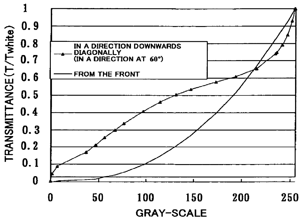
FIG. 2 (PRIOR ART)
