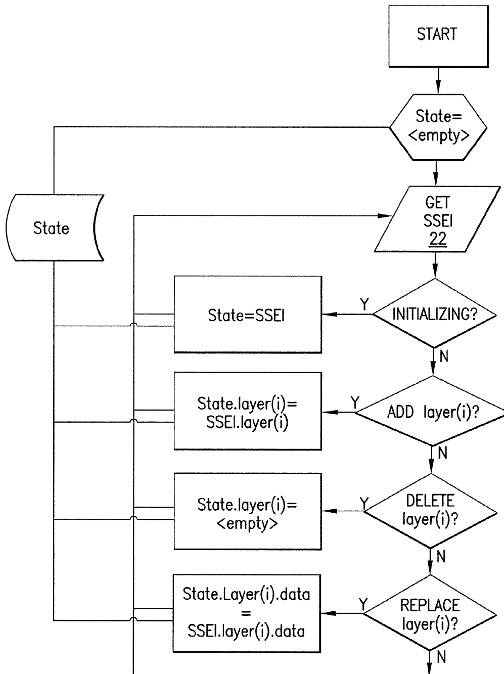
STATE PROCESSING FLOW DIAGRAM 200
