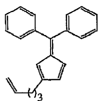
2-(pent-4-enyl)-6,6-diphenylpentafulvene
