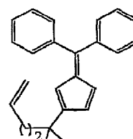
2-(1,1-dimethylpent-4-enyl)-6,6-diphenylpentafulvene
