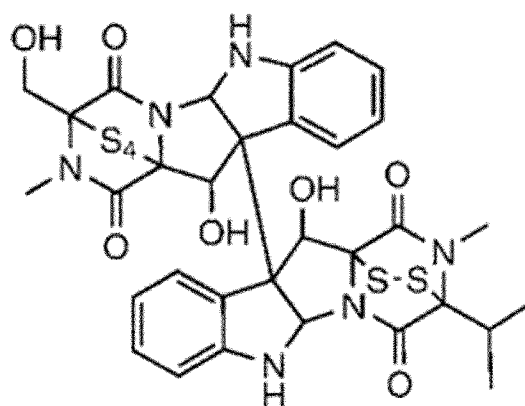
[Chemical Formula 24]
