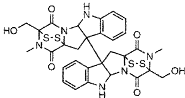
[Chemical Formula 22]
