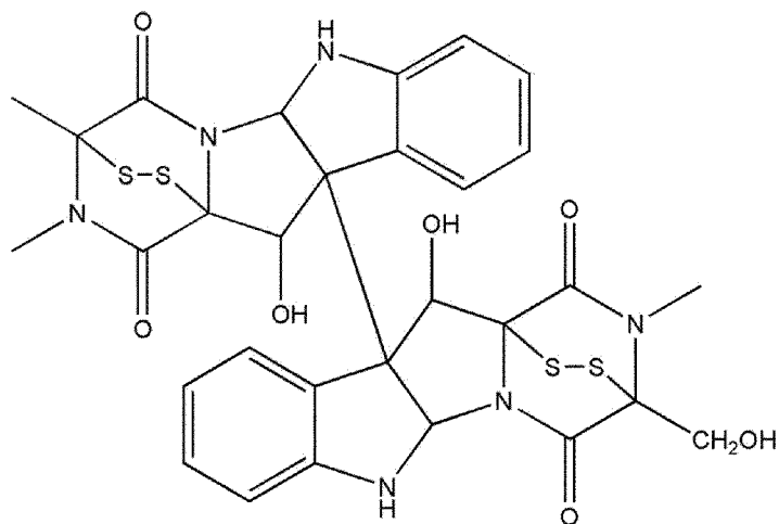
[Chemical Formula 31]
