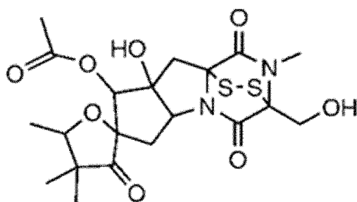
[Chemical Formula 18]
