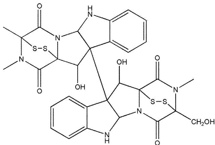
[Chemical Formula 31]
