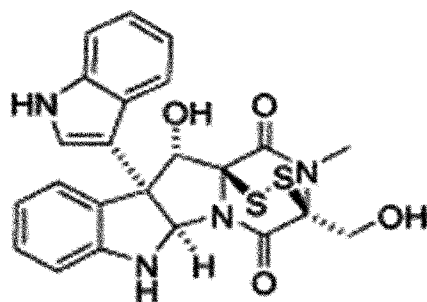
[Chemical Formula 39]
