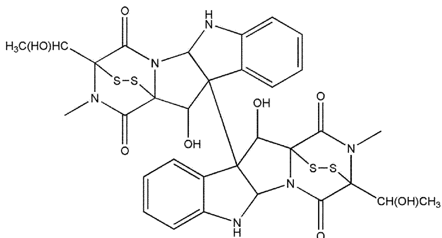
[Chemical Formula 31]
