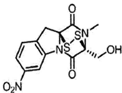
[Chemical Formula 33]
