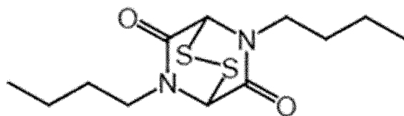
[Chemical Formula 14]
