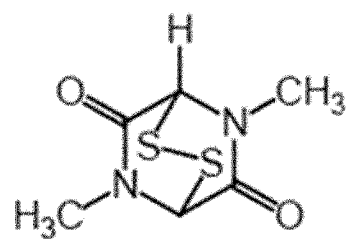
[Chemical Formula 8]
