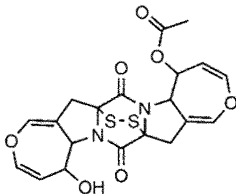
[Chemical Formula 29]
