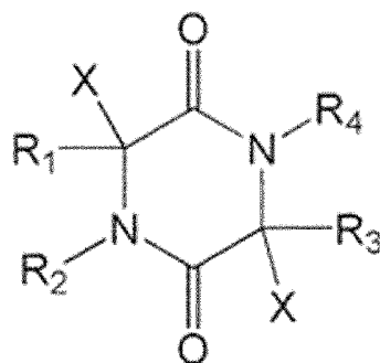
[Chemical Formula 6]
