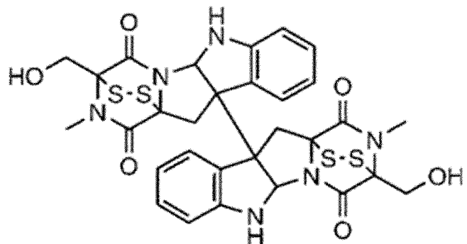
[Chemical Formula 21]
