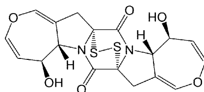
[Chemical Formula 40]
