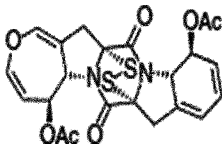
[Chemical Formula 37]
