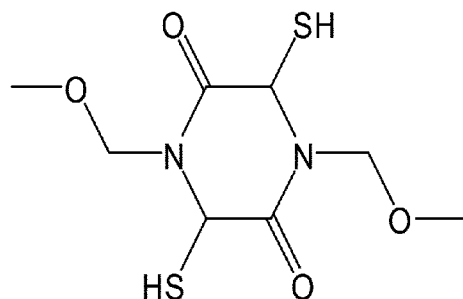
[Chemical Formula 45]
