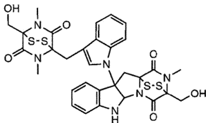
[Chemical Formula 20]
