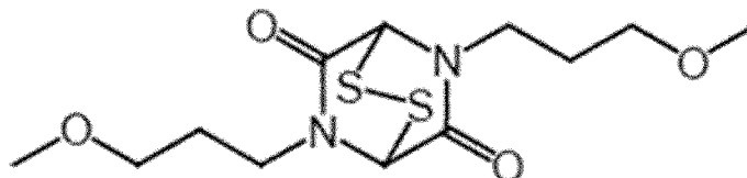
[Chemical Formula 15]
