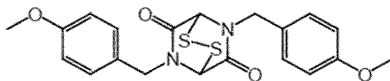
[Chemical Formula 10]
