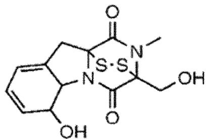
[Chemical Formula 17]
