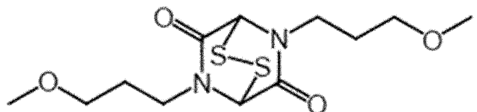
[Chemical Formula 14]
