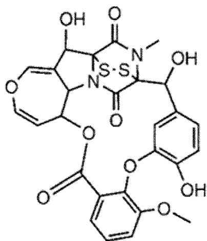
[Chemical Formula 25]
