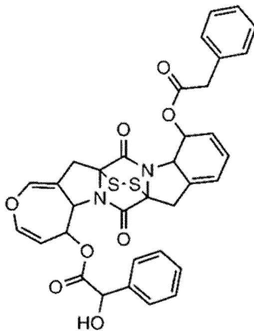
[Chemical Formula 30]
