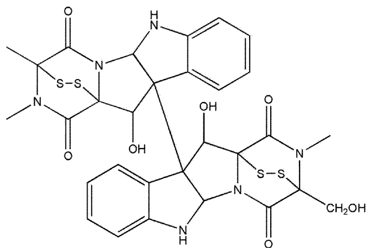
[Chemical Formula 31]
