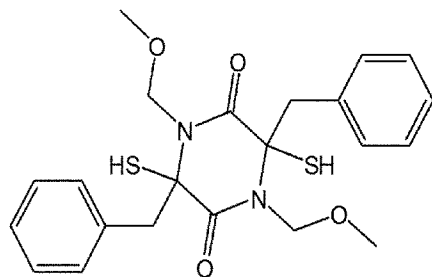
[Chemical Formula 44]
