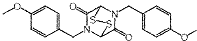
[Chemical Formula 10]
