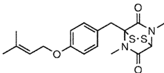
[Chemical Formula 27]
