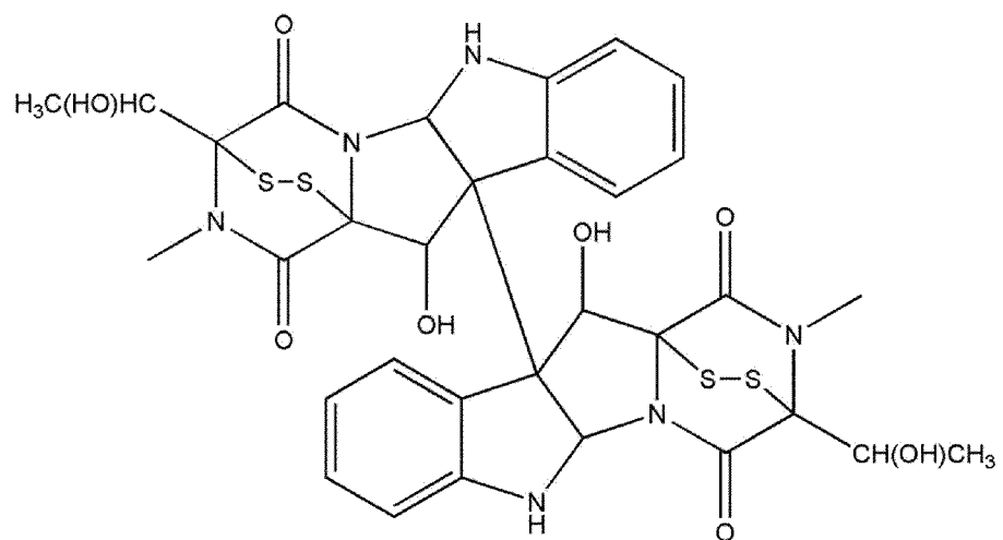
[Chemical Formula 32]
