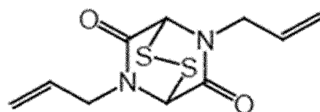
[Chemical Formula 11]
