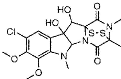
[Chemical Formula 20]
