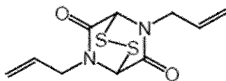
[Chemical Formula 11]
