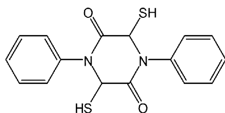
[Chemical Formula 46]
