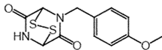
[Chemical Formula 12]
