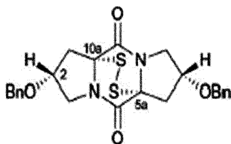
[Chemical Formula 35]
