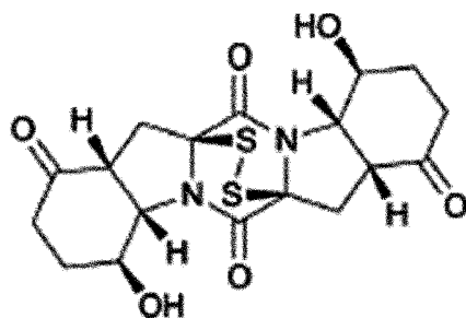
[Chemical Formula 34]
