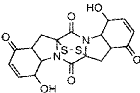
[Chemical Formula 28]
