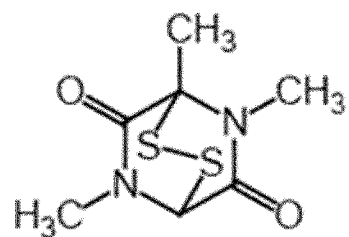
[Chemical Formula 9]
