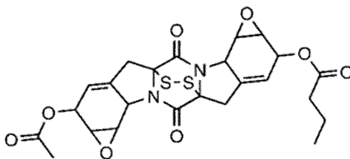
[Chemical Formula 26]
