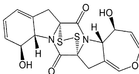
[Chemical Formula 42]
