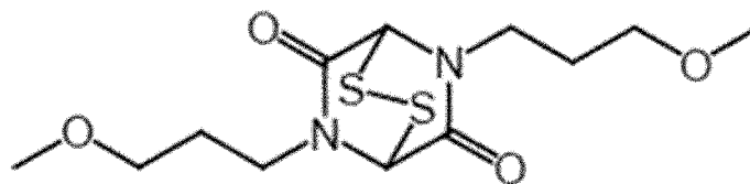
[Chemical Formula 15]
