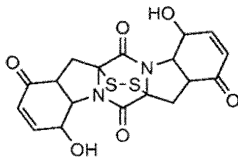
[Chemical Formula 28]
