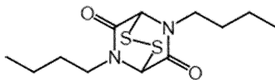
[Chemical Formula 14]
