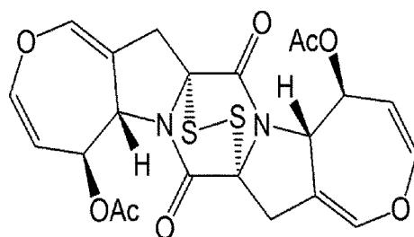
[Chemical Formula 41]
