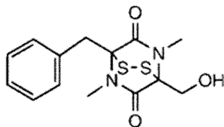
[Chemical Formula 19]
