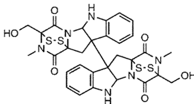
[Chemical Formula 22]
