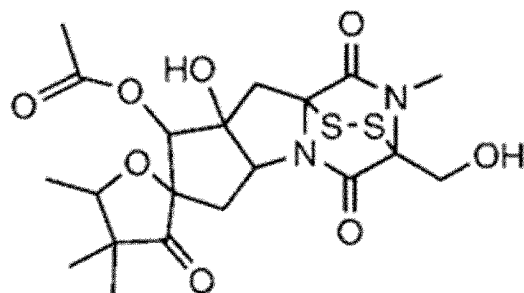
[Chemical Formula 18]
