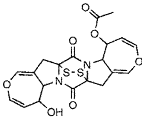
[Chemical Formula 29]
