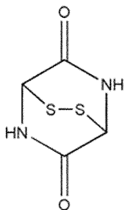
[Chemical Formula 17]
