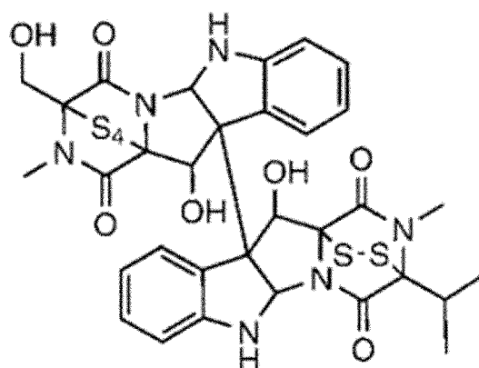
[Chemical Formula 24]
