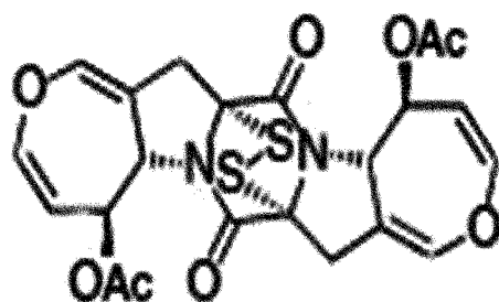
[Chemical Formula 36]
