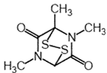
[Chemical Formula 9]
