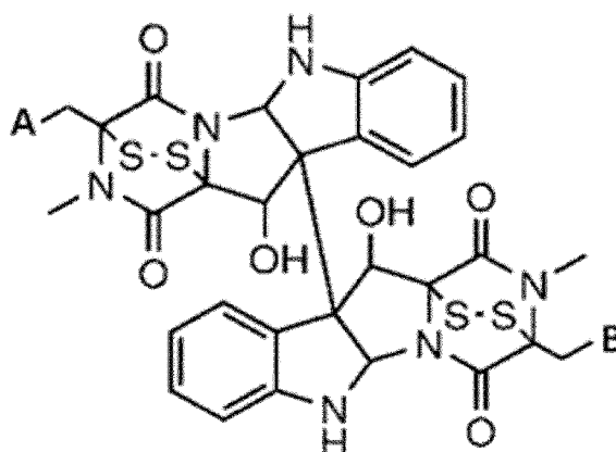
[Chemical Formula 22]
