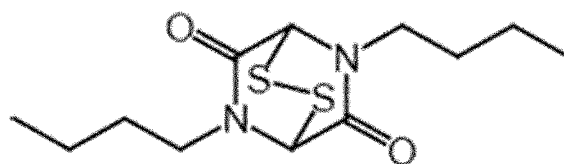
[Chemical Formula 14]
