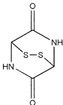
[Chemical Formula 16]
