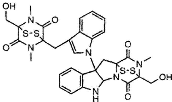
[Chemical Formula 21]
