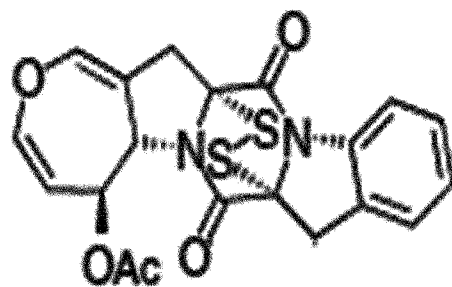
[Chemical Formula 37]
