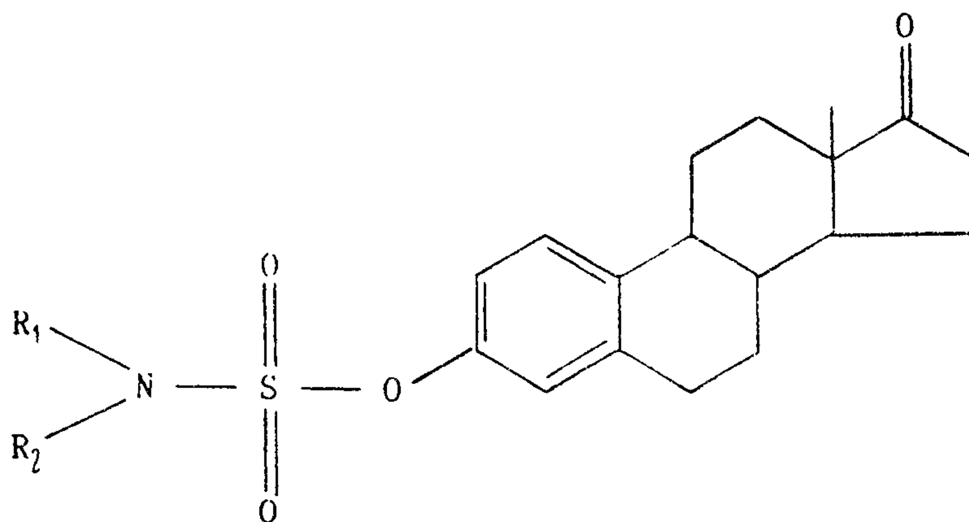
FORMULA (III)
