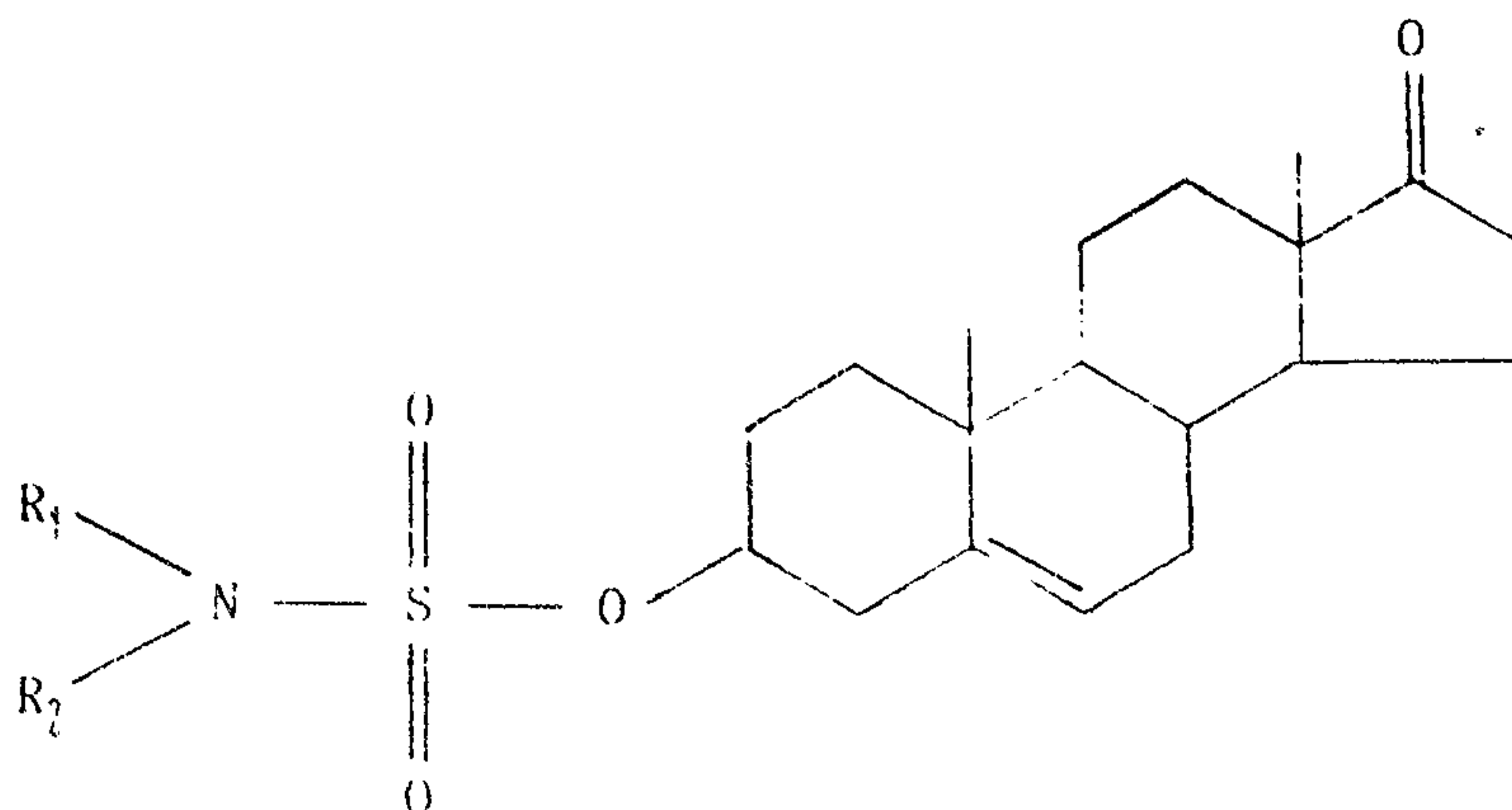
FORMULA (IV)
