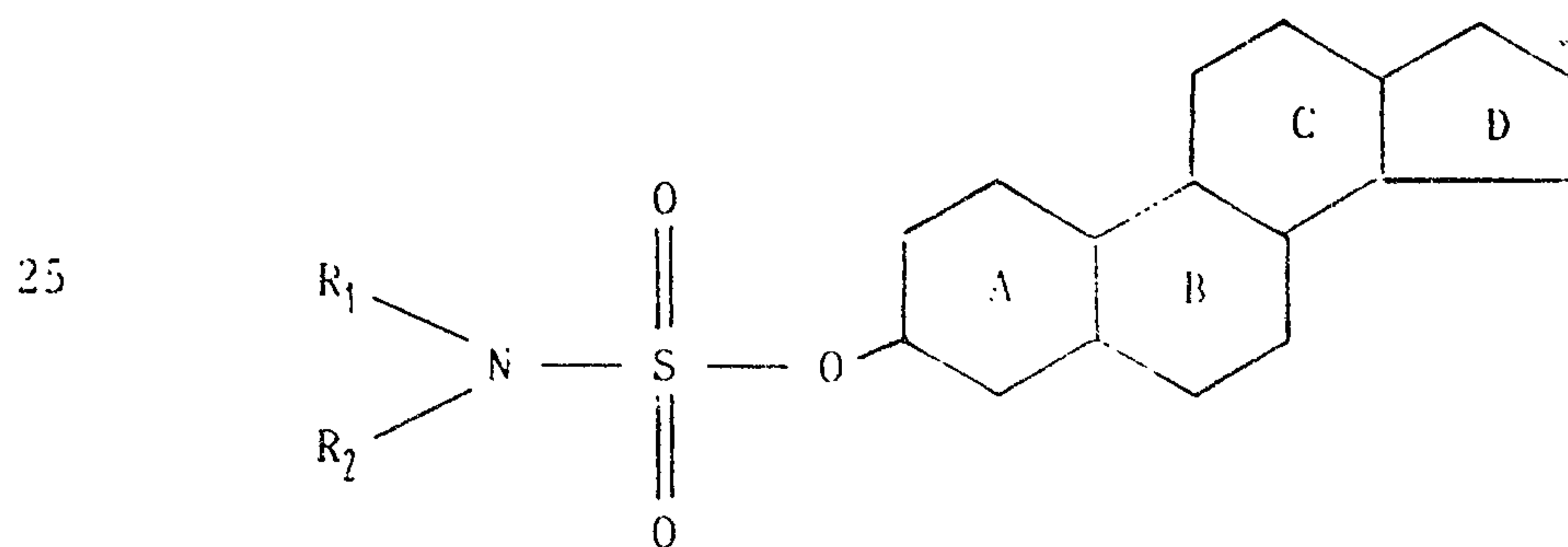
FORMULA (II)
