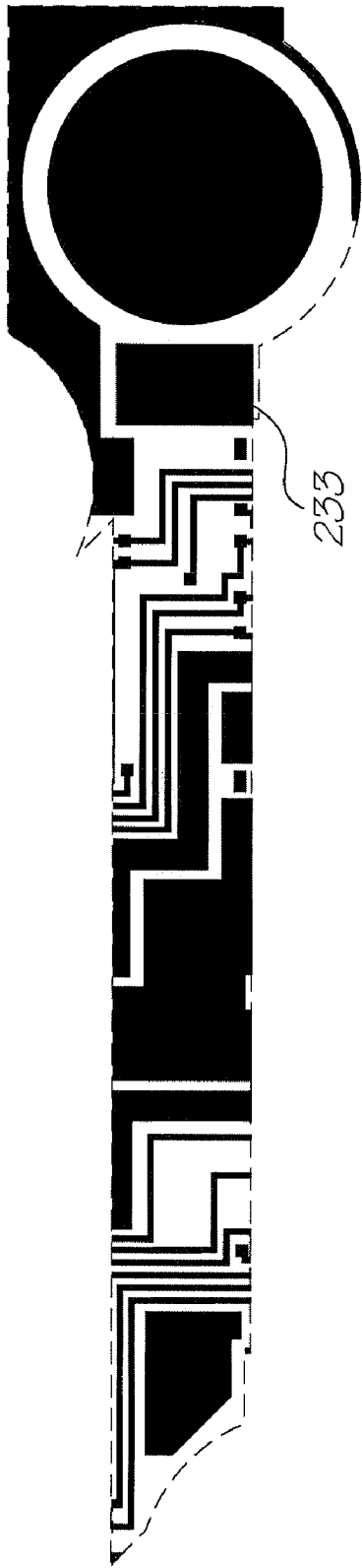
Metal 2 mask
