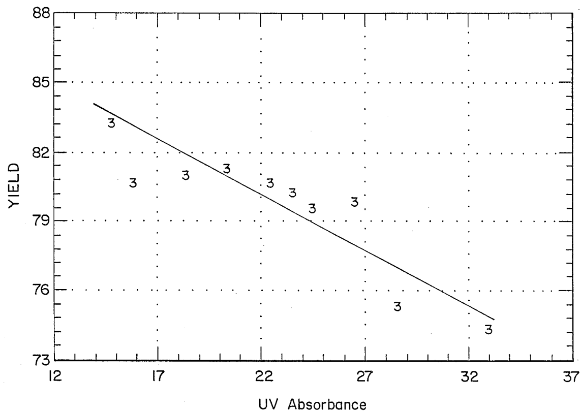
Plot of UV Absorbance vs Yield
