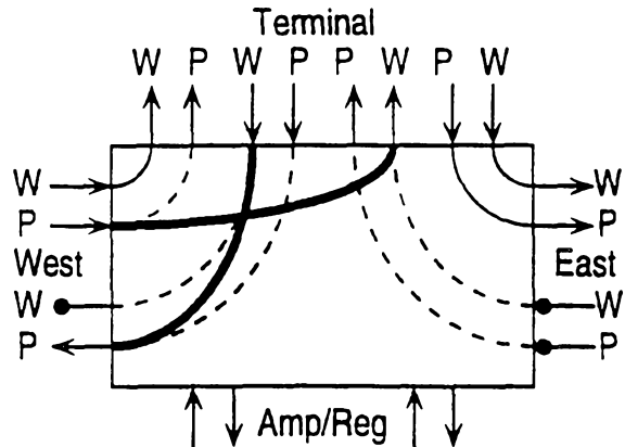
(iii) 10. Ring Switch West-In. Span Switch West-Out
