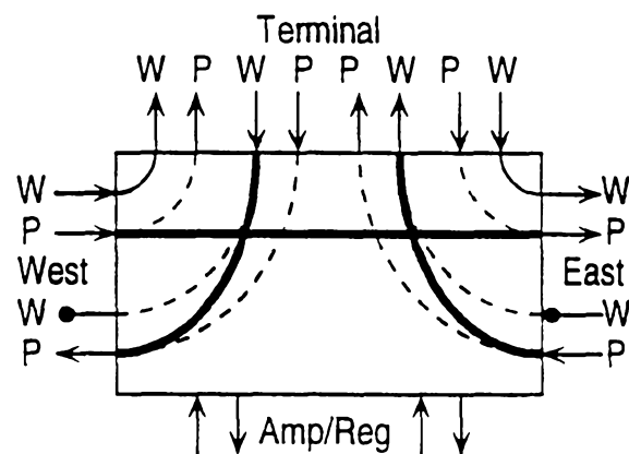
(iv) 4. P-Transit West-to-East, Span Switch West-Out, East-In
