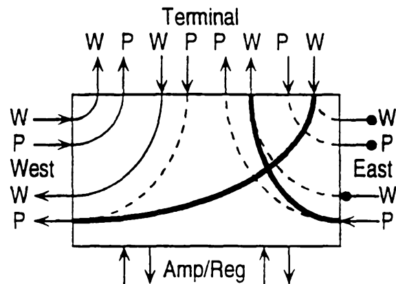
(iii) 12. Ring Switch West-Out. Span Switch East-In
