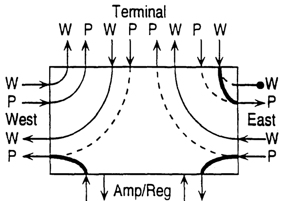
(iv) 16. P-Transit (Amp/Regen) East-to-West. Span Switch East-Out
