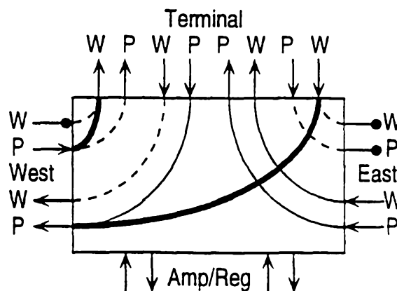
(iii) 13. Ring Switch West-Out. Span Switch West-In
