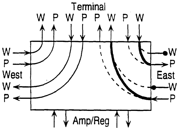
(ii) 6. Span Switch East-In, East-Out
