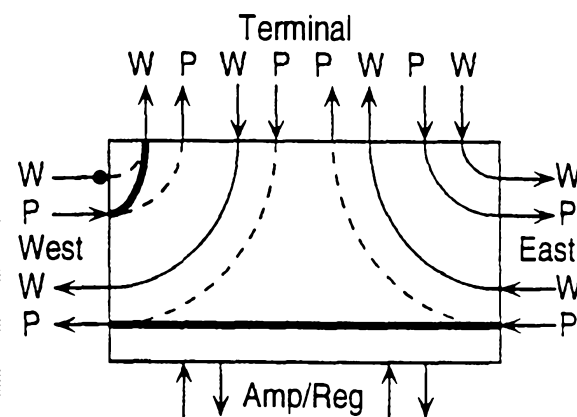
(iv) 6. P-Transit East-to-West, Span Switch West-In
