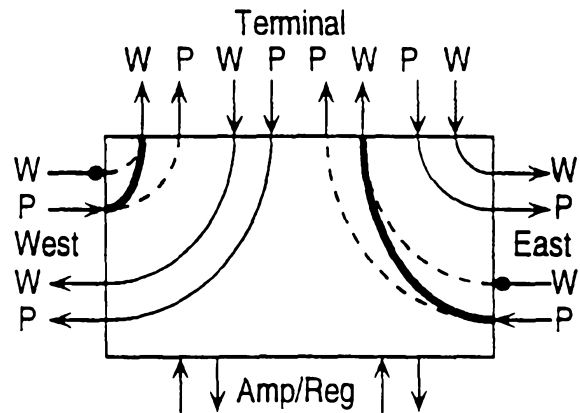
(ii) 9. Span Switch West-In, East-In
