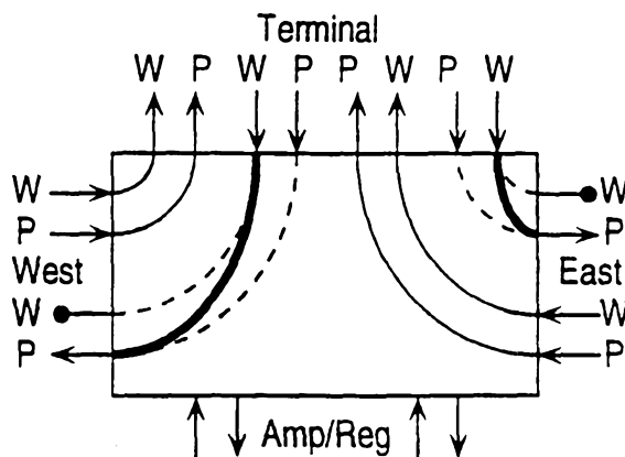
(ii) 10. Span Switch West-Out, East-Out
