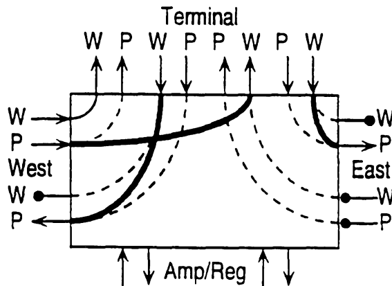
(iii) 11. Ring Switch West-In. Span Switch East-Out, West-Out
