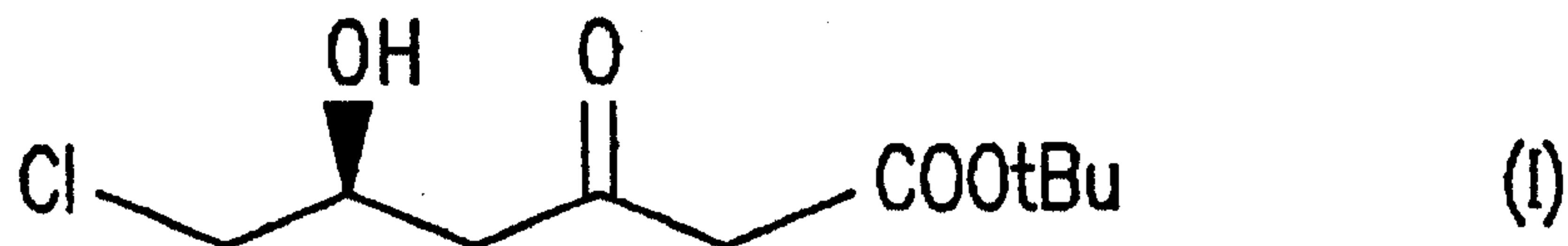
tert-butyl (S)-6-chloro-5-hydroxy-3-oxohexanoate
