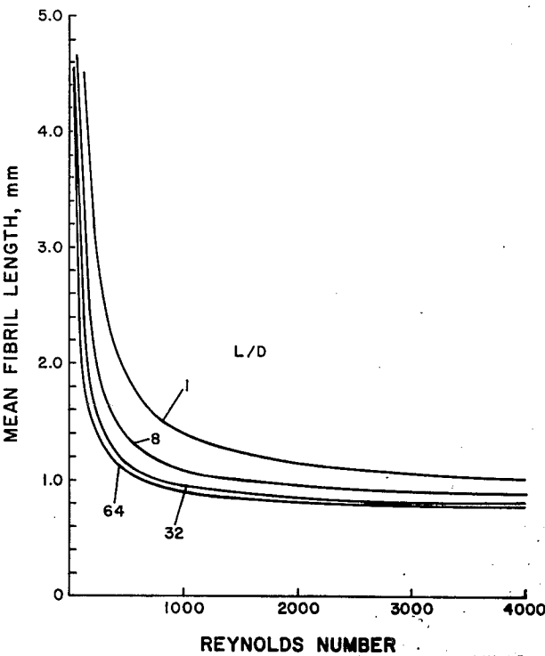
MEAN FIBRIL LENGTH VERSUS REYNOLDS NUMBER AND RATIO OF LENGTH TO INTERNAL DIAMETER OF DISCHARGE MEANS
