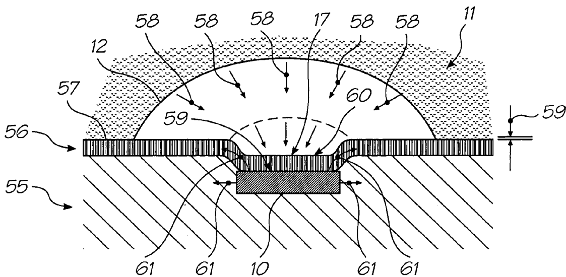
FIG. 47 (PRIOR ART)
