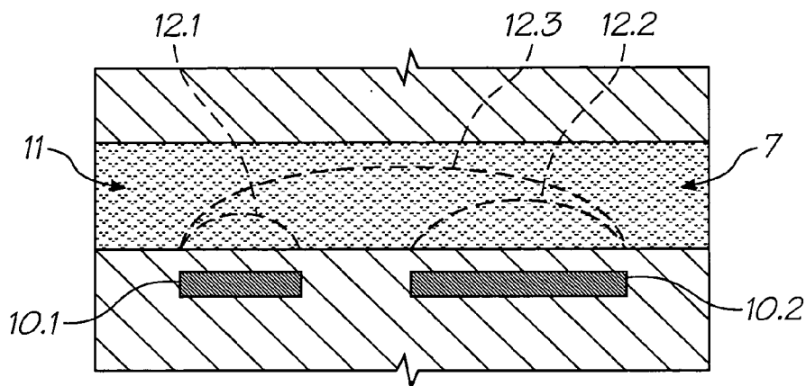
FIG. 52 (PRIOR ART)
