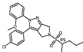
Cpd 41
