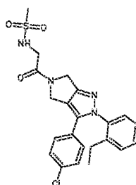
Cpd 12
