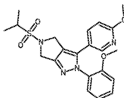
Cpd 97
