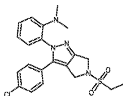
Cpd 89
