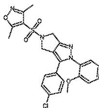
Cpd 87
