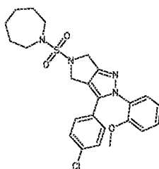
Cpd 55
