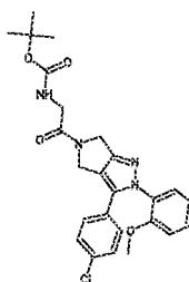
Cpd 29
