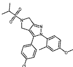
Cpd 67
