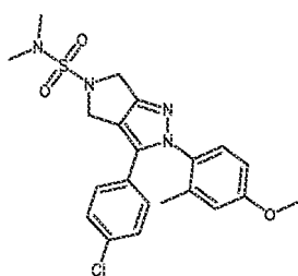
Cpd 69
