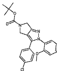
Cpd 28
