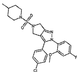
Cpd 73
