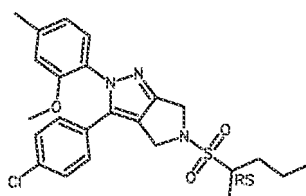
Cpd 76
