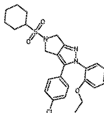
Cpd 52
