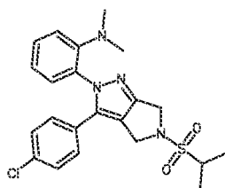
Cpd 88
