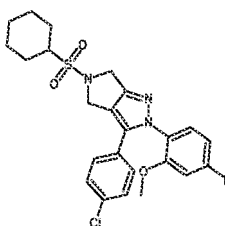
Cpd 72
