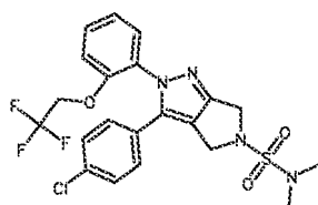
Cpd 90
