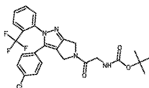
Cpd 18
