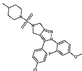
Cpd 80
