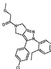
Cpd 10
