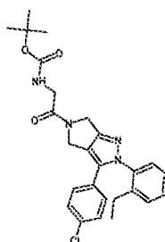
Cpd 11
