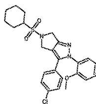
Cpd 37
