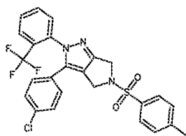
Cpd 17
