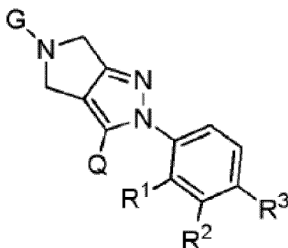
Formel (I),
