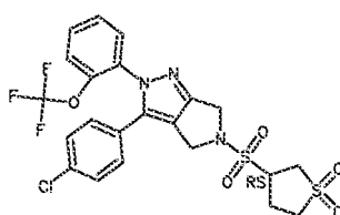
Cpd 48
