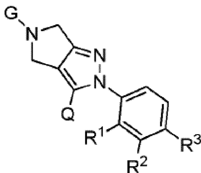
Formel (I),
