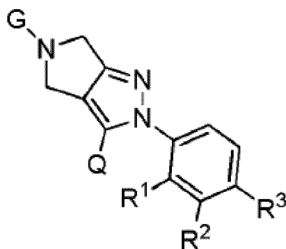
Formel (I),
