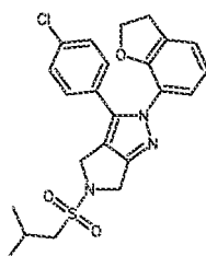
Cpd 85
