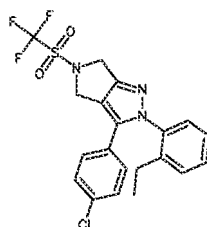
Cpd 3
