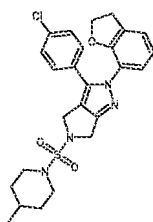
Cpd 86
