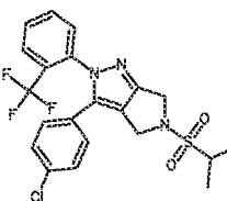
Cpd 16
