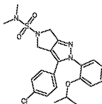
Cpd 63
