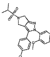
Cpd 31
