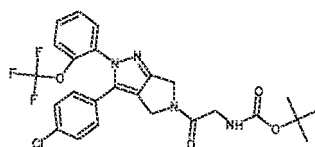
Cpd 22
