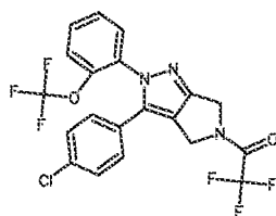
Cpd 21
