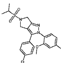
Cpd 75
