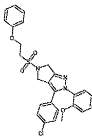
Cpd 43
