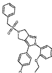
Cpd 53
