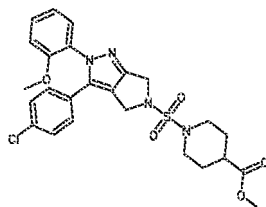
Cpd 58
