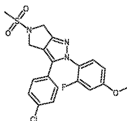
Cpd 78
