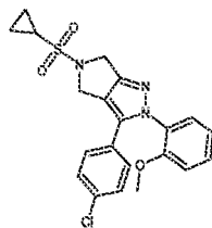
Cpd 32
