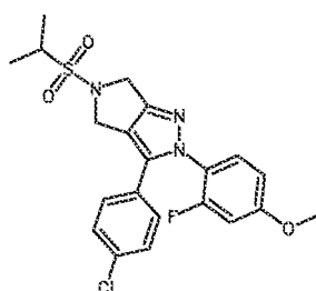
Cpd 79
