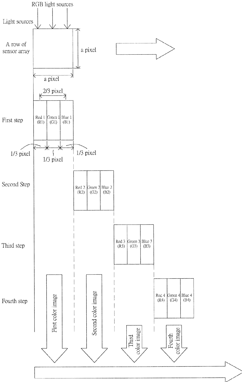
FIG.5 (PRIOR ART)
