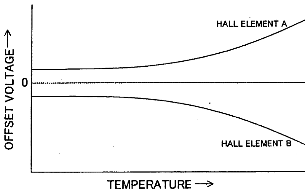
OFFSET VOLTAGE - TEMPERATURE CHARACTERISTIC OF HALL ELEMENT (DRIVING AT CONSTANT CURRENT)
