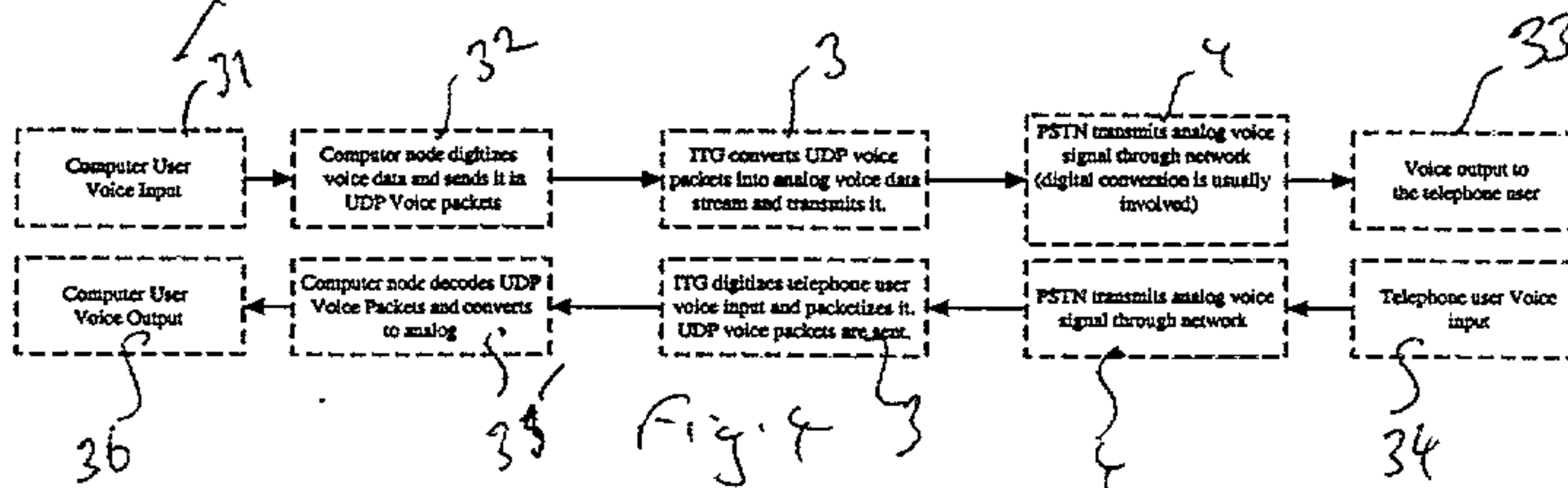
DIAGRAM D: Speech path - how voice transmission is achieved between the computer user and telephone user. This path is established at call setup time and remains in place until call teardown.
