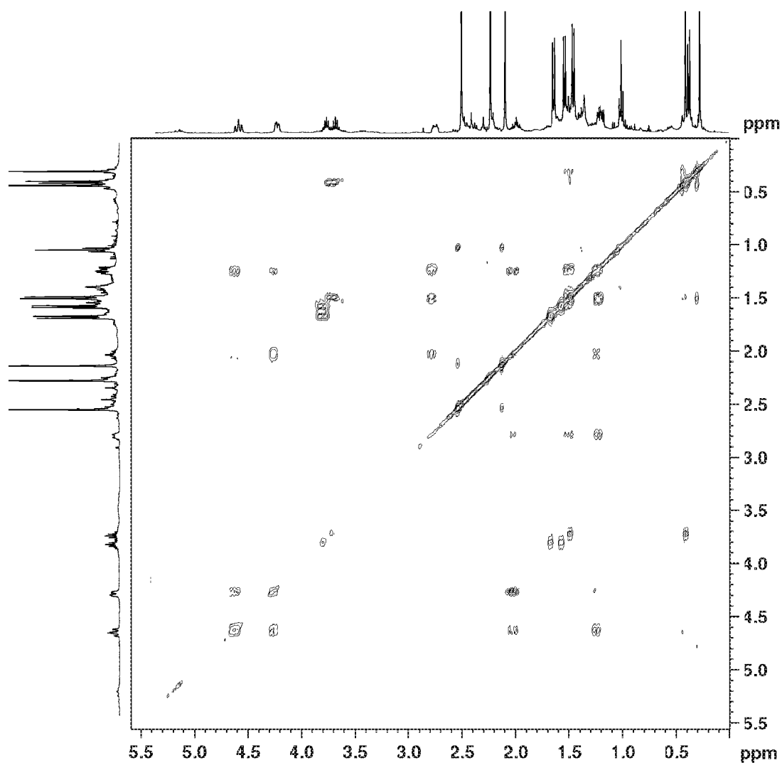
Figure 6. COSY NMR Spectrum for Snap-Shut Catalyst
