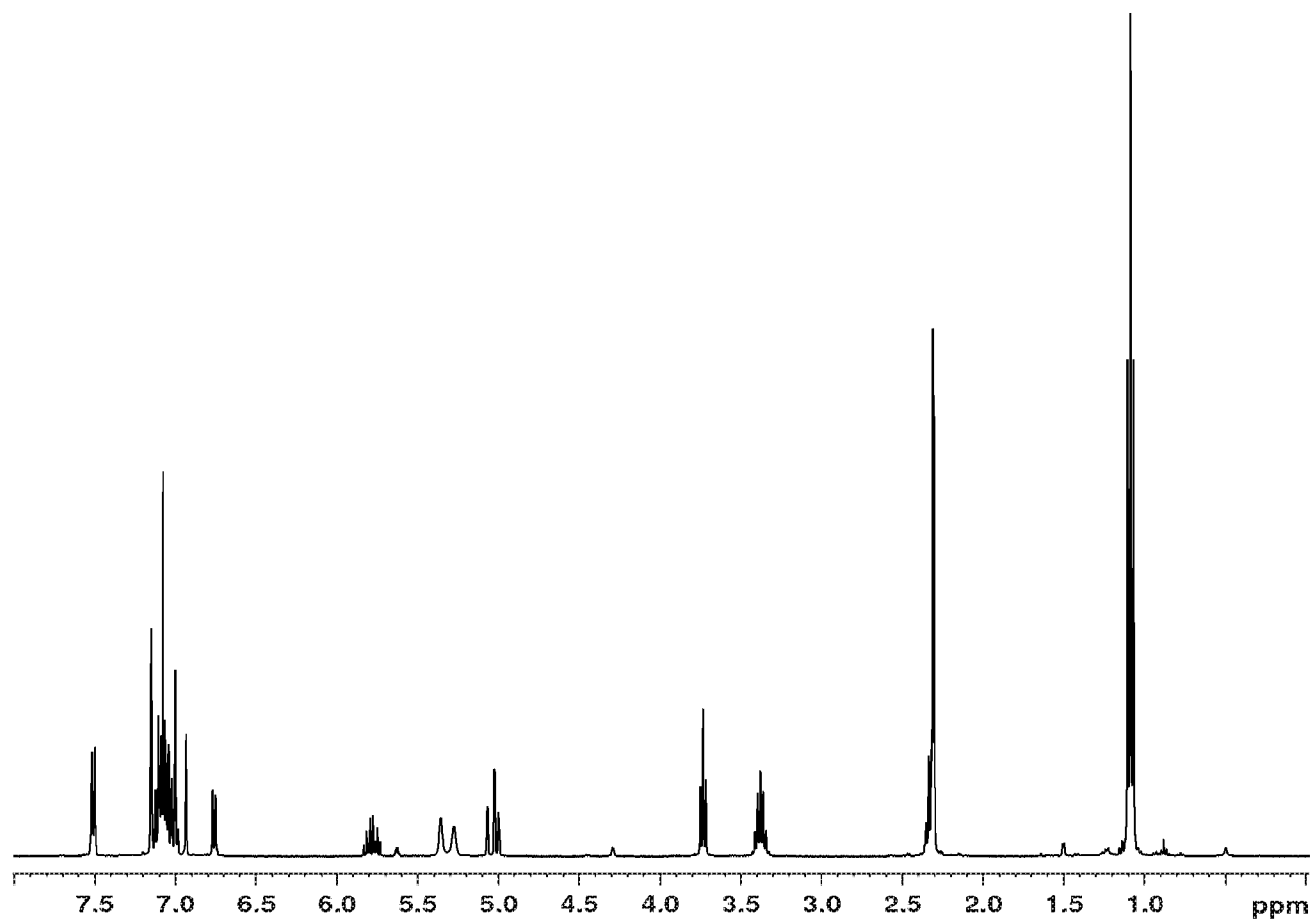
Figure 1. ^1\text{H} NMR for N-((6-(5-(But-3-enyloxy)-2,4-dimethylphenyl)pyridin-2-yl)(phenyl)methyl)-2,6-diisopropylaniline.
