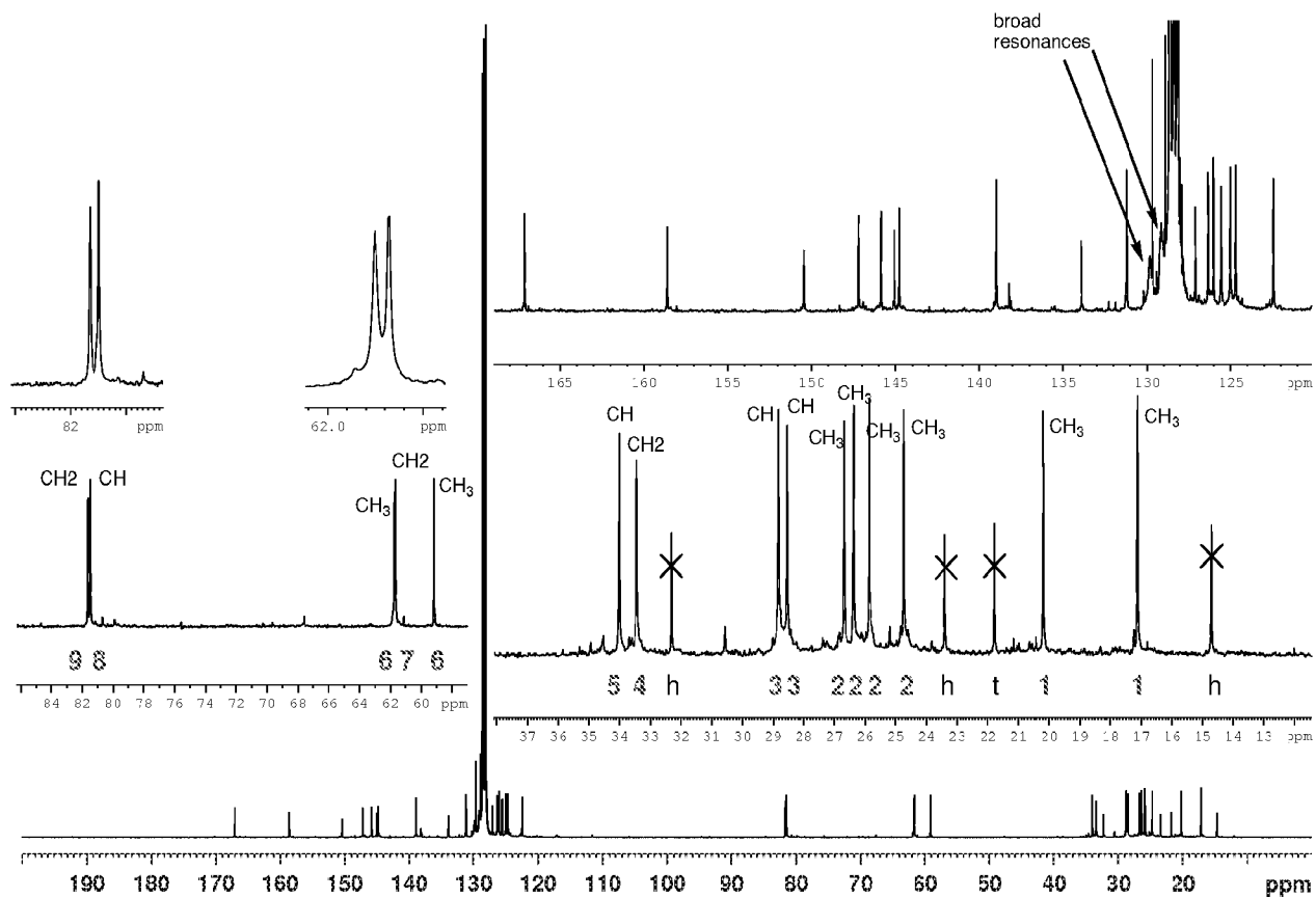
Figure 4. ^{13}\text{C} NMR of Snap-Shut Catalyst. Refer to Figure 5 for ^{13}\text{C} assignments. h = hexane; t = toluene.
