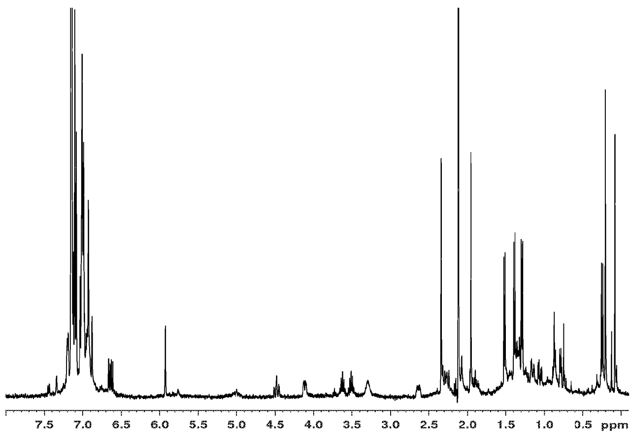
Figure 3. ^1\text{H} NMR of "Snap-Shut" Catalyst
