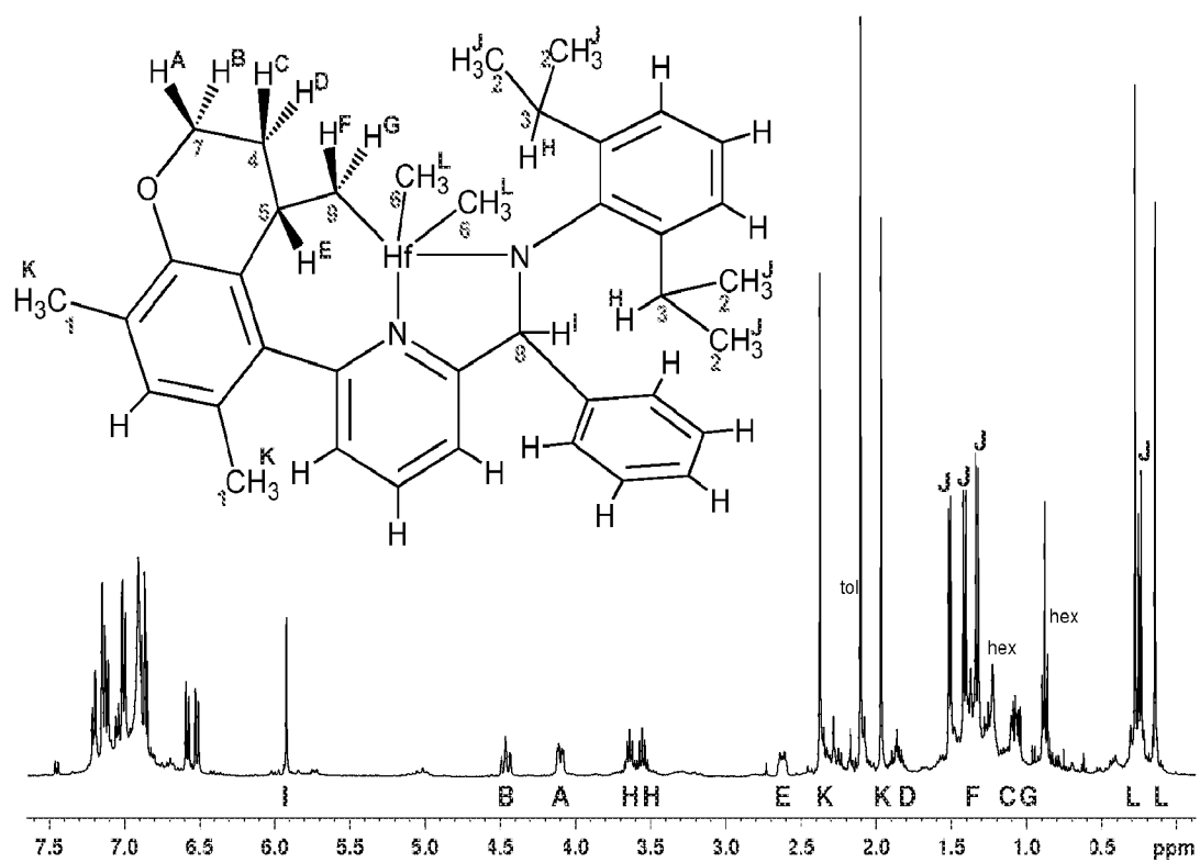
Figure 5. ^1\text{H} NMR with assignments of selected signals.
