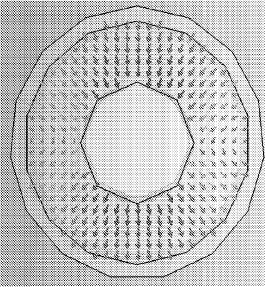
HE11, Horizontal Polarization
