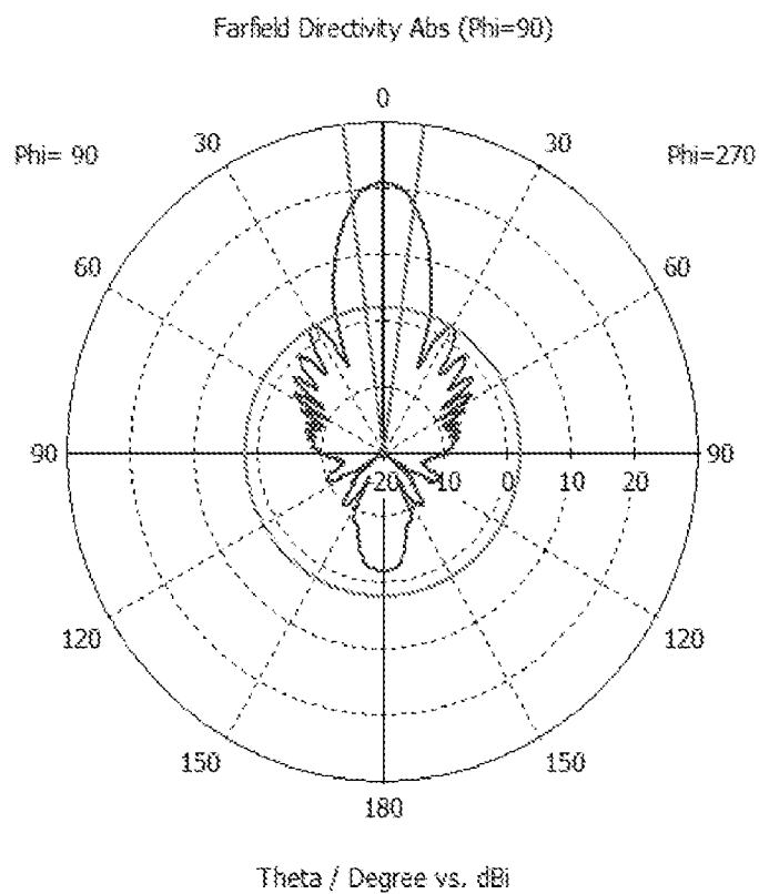
Antenna Gain Pattern
