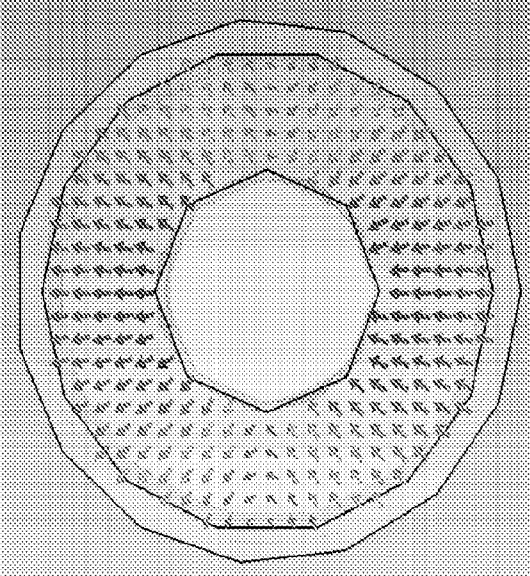
HE11, Vertical Polarization
