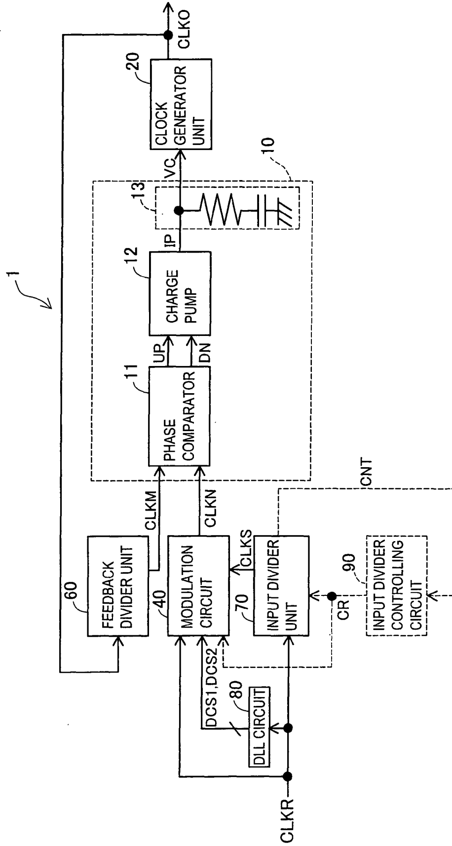
FIG. 1 CIRCUIT BLOCK DIAGRAM OF A SPREAD SPECTRUM CLOCK GENERATION CIRCUIT 1
