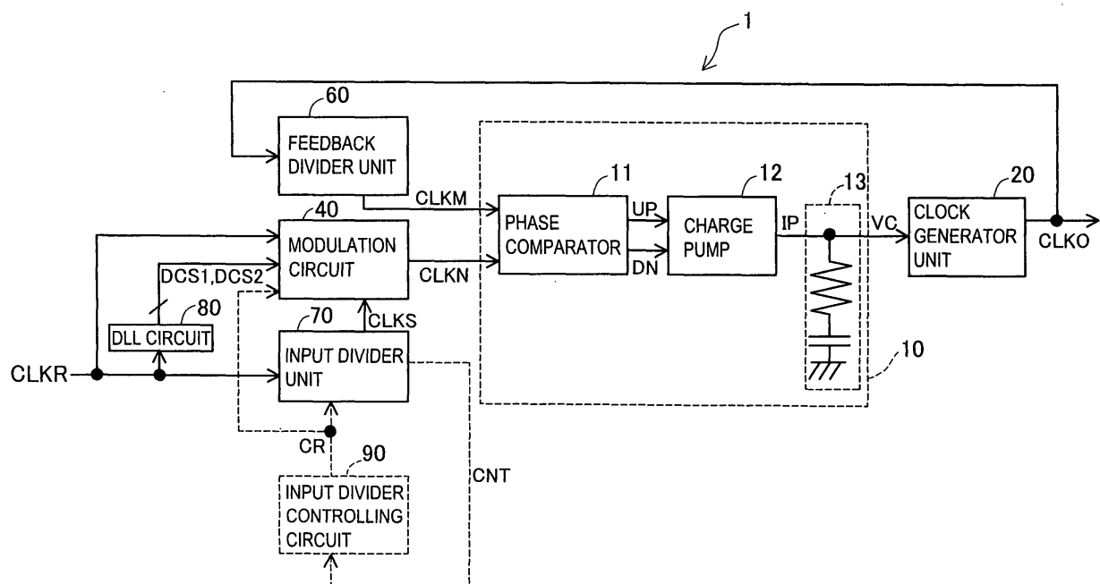
FIG. 1 CIRCUIT BLOCK DIAGRAM OF A SPREAD SPECTRUM CLOCK GENERATION CIRCUIT 1
