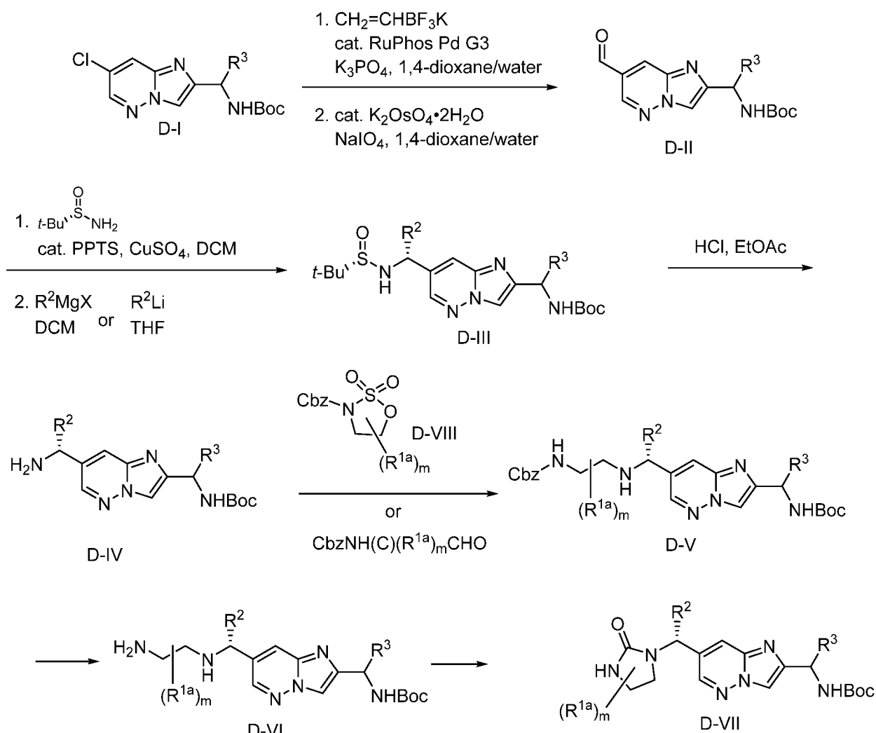
Scheme 3
