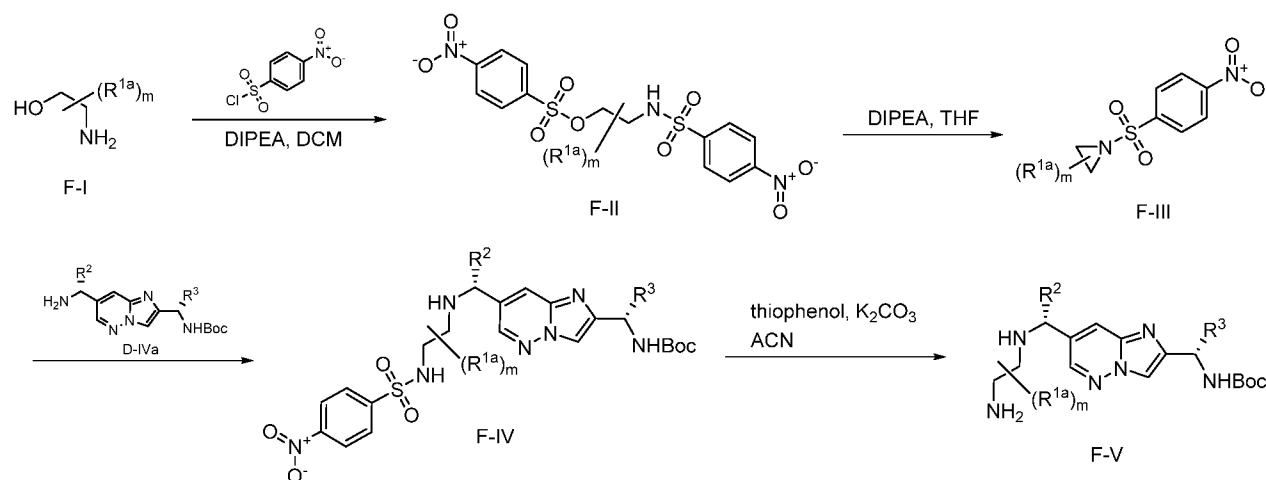
Scheme 6
