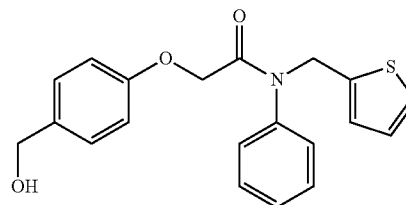
2-(4-(hydroxymethyl)phenoxy)-N-phenyl-N-(thiophen-2-ylmethyl) acetamide
