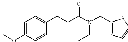
N-ethyl-3-(4-methoxyphenyl)-N-(thiophen-2-ylmethyl)propanamide
