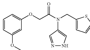
2-(3-methoxyphenoxy)-N-(1H-pyrazol-4-yl)-N-(thiophen-2-ylmethyl)acetamide
