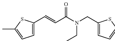
(E)-N-ethyl-3-(5-methylthiophen-2-yl)-N-(thiophen-2-ylmethyl)acrylamide
