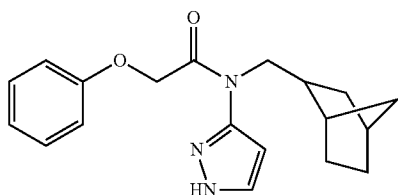
N-(bicyclo[2.2.1]heptan-2-ylmethyl)-2-phenoxy-N-(1H-pyrazol-3-yl)acetamide
