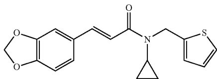
(E)-3-(benzo[d][1,3]dioxol-5-yl)-N-cyclopropyl-N-(thiophen-2-ylmethyl)acrylamide
