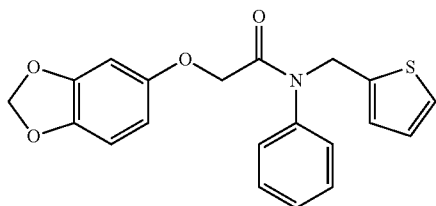
2-(benzo[d][1,3]dioxol-5-yloxy)-N-phenyl-N-(thiophen-2-ylmethyl)acetamide
