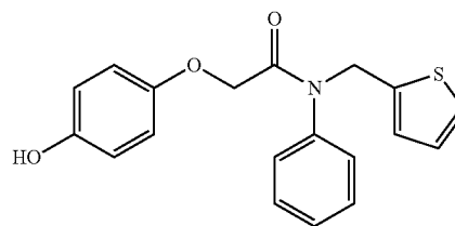
2-(4-hydroxyphenoxy)-N-phenyl-N-(thiophen-2-ylmethyl)acetamide
