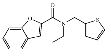
N-ethyl-N-(thiophen-2-ylmethyl)benzofuran-2-carboxamide
