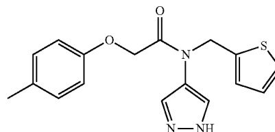
N-(1H-pyrazol-4-yl)-N-(thiophen-2-ylmethyl)-2-(p-tolyloxy)acetamide
