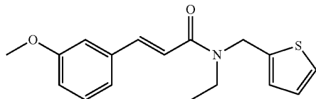
(E)-N-ethyl-3-(3-methoxyphenyl)-N-(thiophen-2-ylmethyl)acrylamide
