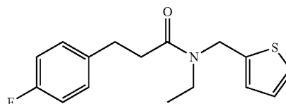
N-ethyl-3-(4-fluorophenyl)-N-(thiophen-2-ylmethyl)propanamide
