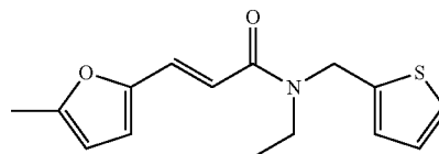
(E)-N-ethyl-3-(5-methylfuran-2-yl)-N-(thiophen-2-ylmethyl)acrylamide
