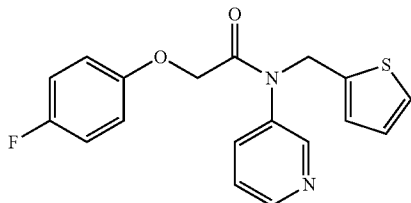
2-(4-fluorophenoxy)-N-(pyridin-3-yl)-N-(thiophen-2-ylmethyl)acetamide
