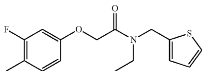
N-ethyl-2-(3-fluoro-4-methylphenoxy)-N-(thiophen-2-ylmethyl)acetamide
