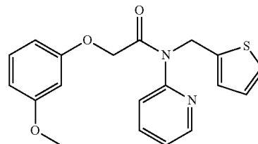
2-(3-methoxyphenoxy)-N-(pyridin-2-yl)-N-(thiophen-2-ylmethyl)acetamide
