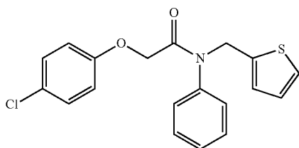
2-(4-chlorophenoxy)-N-phenyl-N-(thiophen-2-ylmethyl)acetamide
