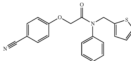
2-(4-cyanophenoxy)-N-phenyl-N-(thiophen-2-ylmethyl)acetamide
