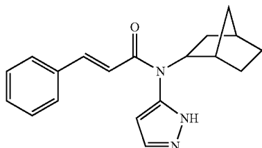
N-(bicyclo[2.2.1]heptan-2-yl)-N-(1H-pyrazol-5-yl) cinnamamide
