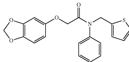
2-(benzo[d][1,3]dioxol-5-yloxy)-N-phenyl-N-(thiophen-2-ylmethyl)acetamide
