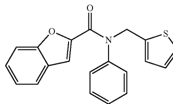
N-phenyl-N-(thiophen-2-ylmethyl)benzofuran-2-carboxamide
