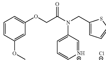
3-(2-(3-methoxyphenoxy)-N-(thiophen-2-ylmethyl)acetamido)pyridinium chloride
