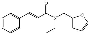
N-ethyl-N-(thiophen-2-ylmethyl)cinnamamide
