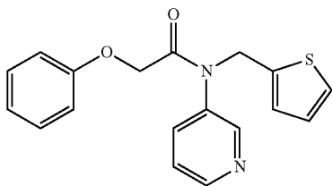
2-phenoxy-N-(pyridin-3-yl)-N-(thiophen-2-ylmethyl)acetamide
