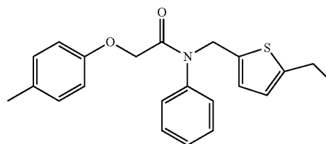
N-((5-ethylthiophen-2-yl)methyl)-N-phenyl-2-(p-tolyloxy)acetamide
