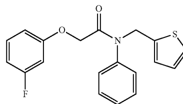
2-(3-fluorophenoxy)-N-phenyl-N-(thiophen-2-ylmethyl)acetamide
