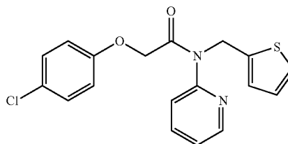
2-(4-chlorophenoxy)-N-(pyridin-2-yl)-N-(thiophen-2-ylmethyl)acetamide
