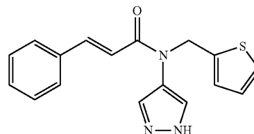
N-(1H-pyrazol-4-yl)-N-(thiophen-2-ylmethyl)cinnamamide
