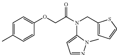
N-(1-methyl-1H-pyrazol-5-yl)-N-(thiophen-2-ylmethyl)-2-(p-tolyloxy)acetamide
