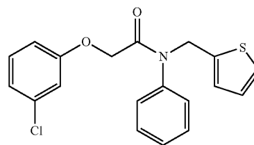
2-(3-chlorophenoxy)-N-phenyl-N-(thiophen-2-ylmethyl)acetamide
