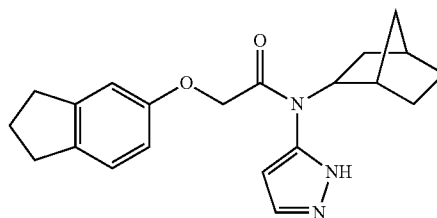
N-(bicyclo[2.2.1]heptan-2-yl)-2-(2,3-dihydro-1H-inden-5-yloxy)-N-(1H-pyrazol-5-yl)acetamide
