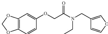
2-(benzo[d][1,3]dioxol-5-yloxy)-N-ethyl-N-(furan-3-ylmethyl)acetamide
