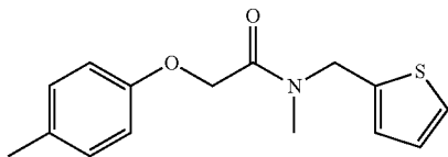
N-methyl-N-(thiophen-2-ylmethyl)-2-(p-tolyloxy)acetamide
