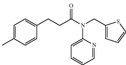
N-(pyridin-2-yl)-N-(thiophen-2-ylmethyl)-3-p-tolyl- propanamide
