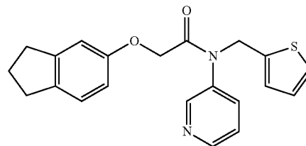
2-(2,3-dihydro-1H-inden-5-yloxy)-N-(pyridin-3-yl)-N-(thiophen-2-ylmethyl)acetamide
