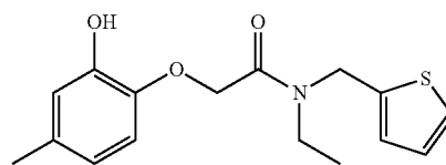
N-ethyl-2-(2-hydroxy-4-methylphenoxy)-N-(thiophen-2-ylmethyl)acetamide
