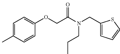
N-propyl-N-(thiophen-2-ylmethyl)-2-(p-tolyloxy) acetamide
