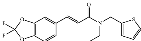
(E)-3-(2,2-difluorobenzo[d][1,3]dioxol-5-yl)-N-ethyl-N-(thiophen-2-ylmethyl)acrylamide
