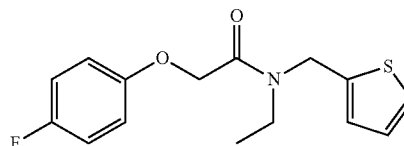
N-ethyl-2-(4-fluorophenoxy)-N-(thiophen-2-ylmethyl)acetamide
