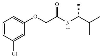
(R)-2-(3-chlorophenoxy)-N-(3-methylbutan-2-yl) acetamide
