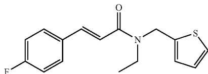
(E)-N-ethyl-3-(4-fluorophenyl)-N-(thiophen-2-ylmethyl)acrylamide
