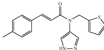
(E)-N-(1H-pyrazol-4-yl)-N-(thiophen-2-ylmethyl)-3-p-tolylacrylamide
