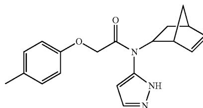
endo/exo mixture
