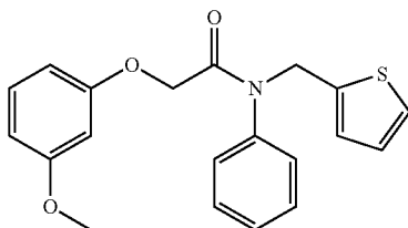
2-(3-methoxyphenoxy)-N-phenyl-N-(thiophen-2-ylmethyl)acetamide
