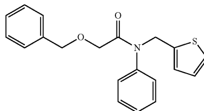
2-(benzyloxy)-N-phenyl-N-(thiophen-2-ylmethyl) acetamide
