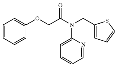
2-phenoxy-N-(pyridin-2-yl)-N-(thiophen-2-ylmethyl)acetamide
