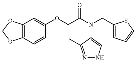
2-(benzo[d][1,3]dioxol-5-yloxy)-N-(3-methyl-1H-pyrazol-4-yl)-N-(thiophen-2-ylmethyl)acetamide
