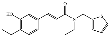
(E)-N-ethyl-3-(3-hydroxy-4-methoxyphenyl)-N-(thiophen-2-ylmethyl)acrylamide
