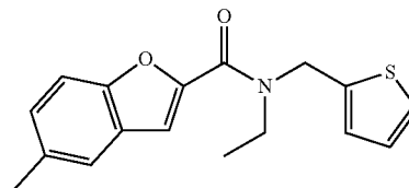
N-ethyl-5-methyl-N-(thiophen-2-ylmethyl)benzofuran-2-carboxamide
