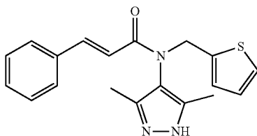
N-(3,5-dimethyl-1H-pyrazol-4-yl)-N-(thiophen-2-ylmethyl)cinnamamide
