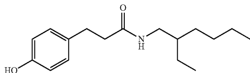
N-(2-ethylhexyl)-3-(4-hydroxyphenyl)propanamide
