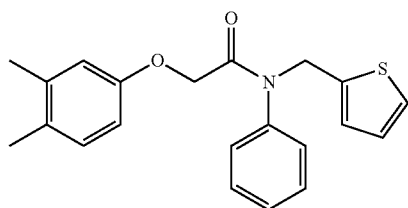
2-(3,4-dimethylphenoxy)-N-phenyl-N-(thiophen-2-ylmethyl)acetamide
