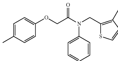
N-((3-methylthiophen-2-yl)methyl)-N-phenyl-2-(p-tolyloxy)acetamide
