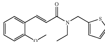
(E)-N-ethyl-3-(2-methoxyphenyl)-N-(thiophen-2-ylmethyl)acrylamide
