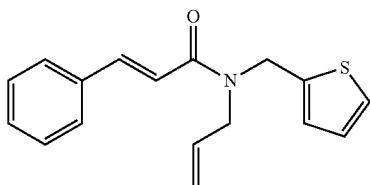
N-allyl-N-(thiophen-2-ylmethyl)cinnamamide
