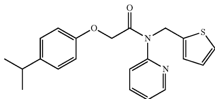
2-(4-isopropylphenoxy)-N-(pyridin-2-yl)-N-(thiophen-2-ylmethyl)acetamide
