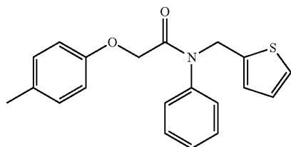
N-phenyl-N-(thiophen-2-ylmethyl)-2-(p-tolyloxy) acetamide
