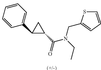
(+/-) (E)-N-ethyl-2-phenyl-N-(thiophen-2-ylmethyl)cyclopropanecarboxamide
