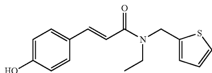
(E)-N-ethyl-3-(4-hydroxyphenyl)-N-(thiophen-2-ylmethyl)acrylamide
