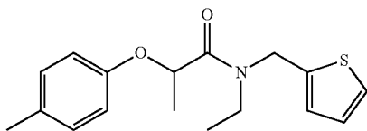
N-ethyl-N-(thiophen-2-ylmethyl)-2-(p-tolyloxy)propanamide
