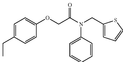
2-(4-ethylphenoxy)-N-phenyl-N-(thiophen-2-ylmethyl)acetamide
