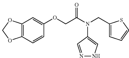
2-(benzo[d][1,3]dioxol-5-yloxy)-N-(1H-pyrazol-4-yl)-N-(thiophen-2-ylmethyl)acetamide
