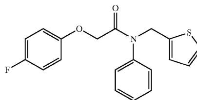
2-(4-fluorophenoxy)-N-phenyl-N-(thiophen-2-ylmethyl)acetamide
