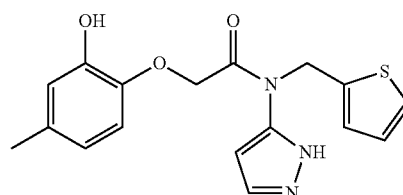
2-(2-hydroxy-4-methylphenoxy)-N-(1H-pyrazol-5-yl)-N-(thiophen-2-ylmethyl)acetamide
