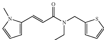
(E)-N-ethyl-3-(1-methyl-1H-pyrrol-2-yl)-N-(thiophen-2-ylmethyl)acrylamide
