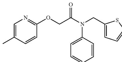
2-(5-methylpyridin-2-yloxy)-N-phenyl-N-(thiophen-2-ylmethyl)acetamide
