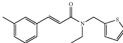
(E)-N-ethyl-N-(thiophen-2-ylmethyl)-3-m-tolylacrylamide
