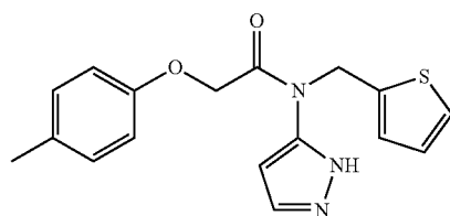
N-(1H-pyrazol-5-yl)-N-(thiophen-2-ylmethyl)-2-(p-tolyloxy)acetamide
