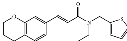
(E)-3-(2,3-dihydrobenzo[b][1,4]dioxin-6-yl)-N-ethyl-N-(thiophen-2-ylmethyl)acrylamide
