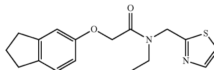
2-(2,3-dihydro-1H-inden-5-yloxy)-N-ethyl-N-(thiazol-5-ylmethyl)acetamide
