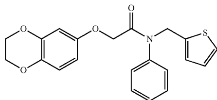
2-(2,3-dihydrobenzo[b][1,4]dioxin-6-yloxy)-N-phenyl-N-(thiophen-2-ylmethyl)acetamide
