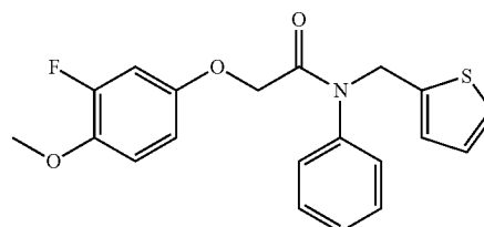
2-(3-fluoro-4-methoxyphenoxy)-N-phenyl-N-(thiophen-2-ylmethyl)acetamide
