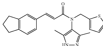
(E)-3-(2,3-dihydro-1H-inden-5-yl)-N-(3,5-dimethyl-1H-pyrazol-4-yl)-N-(thiophen-2-ylmethyl)acrylamide
