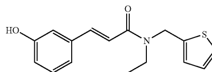
(E)-N-ethyl-3-(3-hydroxyphenyl)-N-(thiophen-2-ylmethyl)acrylamide
