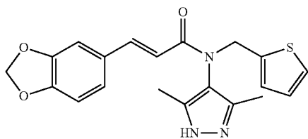
(E)-3-(benzo[d][1,3]dioxol-5-yl)-N-(3,5-dimethyl-1H-pyrazol-4-yl)-N-(thiophen-2-ylmethyl)acrylamide
