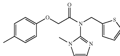
N-(1-methyl-1H-imidazol-2-yl)-N-(thiophen-2-ylmethyl)-2-(p-tolyloxy)acetamide
