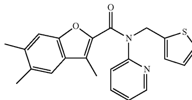
3,5,6-trimethyl-N-(pyridin-2-yl)-N-(thiophen-2-ylmethyl)benzofuran-2-carboxamide
