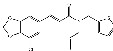
(E)-N-allyl-3-(7-chlorobenzo[d][1,3]dioxol-5-yl)-N-(thiophen-2-ylmethyl)acrylamide
