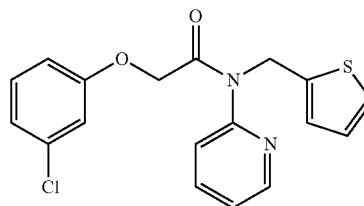
2-(3-chlorophenoxy)-N-(pyridin-2-yl)-N-(thiophen-2-ylmethyl)acetamide
