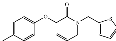
N-allyl-N-(thiophen-2-ylmethyl)-2-(p-tolyloxy)acetamide
