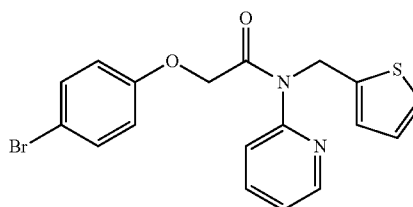
2-(4-bromophenoxy)-N-(pyridin-2-yl)-N-(thiophen-2-ylmethyl)acetamide
