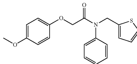
2-(4-methoxyphenoxy)-N-phenyl-N-(thiophen-2-ylmethyl)acetamide
