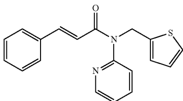
N-(pyridin-2-yl)-N-(thiophen-2-ylmethyl)cinnamamide
