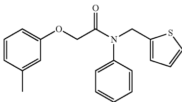
N-phenyl-N-(thiophen-2-ylmethyl)-2-(m-tolyloxy)acetamide
