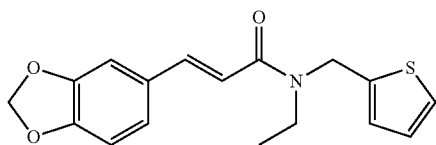
(E)-3-(benzo[d][1,3]dioxol-5-yl)-N-ethyl-N-(thiophen-2-ylmethyl)acrylamide
