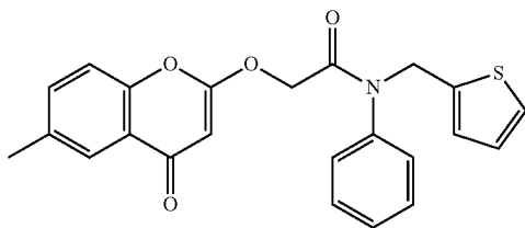
2-(6-methyl-4-oxo-4H-chromen-2-yloxy)-N-phenyl-N-(thiophen-2-ylmethyl)acetamide
