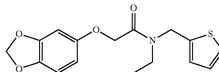
2-(benzo[d][1,3]dioxol-5-yloxy)-N-ethyl-N-(thiophen-2-ylmethyl)acetamide
