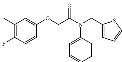
2-(4-fluoro-3-methylphenoxy)-N-phenyl-N-(thiophen-2-ylmethyl)acetamide
