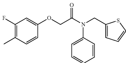
2-(3-fluoro-4-methylphenoxy)-N-phenyl-N-(thiophen-2-ylmethyl)acetamide
