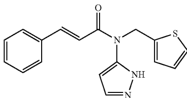
N-(1H-pyrazol-5-yl)-N-(thiophen-2-ylmethyl)cinnamamide
