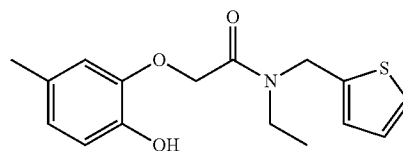
N-ethyl-2-(2-hydroxy-5-methylphenoxy)-N-(thiophen-2-ylmethyl)acetamide
