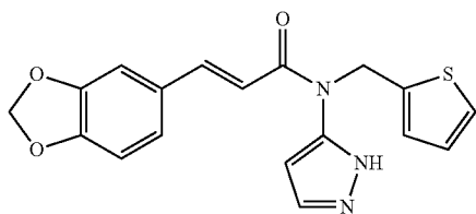
(E)-3-(benzo[d][1,3]dioxol-5-yl)-N-(1H-pyrazol-5-yl)-N-(thiophen-2-ylmethyl)acrylamide
