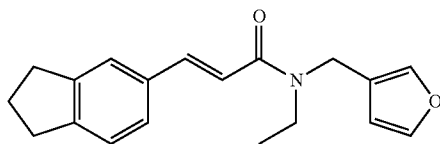
(E)-3-(2,3-dihydro-1H-inden-5-yl)-N-ethyl-N-(furan-3-ylmethyl)acrylamide
