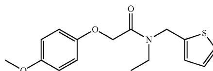
N-ethyl-2-(4-methoxyphenoxy)-N-(thiophen-2-ylmethyl)acetamide
