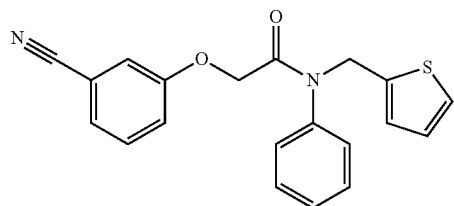
2-(3-cyanophenoxy)-N-phenyl-N-(thiophen-2-ylmethyl)acetamide
