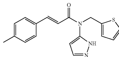
(E)-N-(1H-pyrazol-5-yl)-N-(thiophen-2-ylmethyl)-3-p-tolylacrylamide
