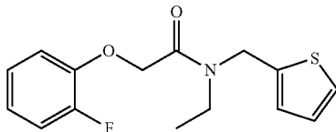
N-ethyl-2-(2-fluorophenoxy)-N-(thiophen-2-ylmethyl) acetamide
