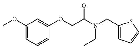
N-ethyl-2-(3-methoxyphenoxy)-N-(thiophen-2-ylmethyl)acetamide
