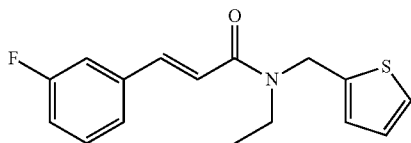
(E)-N-ethyl-3-(3-fluorophenyl)-N-(thiophen-2-ylmethyl)acrylamide
