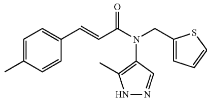
(E)-N-(5-methyl-1H-pyrazol-4-yl)-N-(thiophen-2-ylmethyl)-3-p-tolylacrylamide
