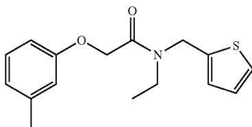
N-ethyl-N-(thiophen-2-ylmethyl)-2-(m-tolyloxy)acetamide
