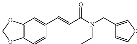
(E)-3-(benzo[d][1,3]dioxol-5-yl)-N-ethyl-N-(furan-3-ylmethyl)acrylamide
