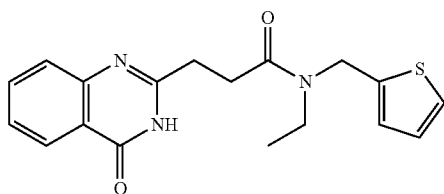
N-ethyl-3-(4-oxo-3,4-dihydroquinazolin-2-yl)-N-(thiophen-2-ylmethyl)propanamide
