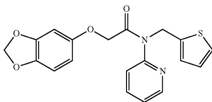
2-(benzo[d][1,3]dioxol-5-yloxy)-N-(pyridin-2-yl)-N-(thiophen-2-ylmethyl)acetamide
