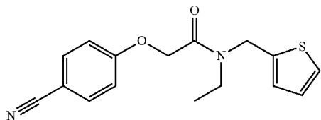
2-(4-cyanophenoxy)-N-ethyl-N-(thiophen-2-ylmethyl)acetamide
