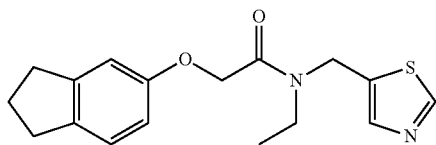
2-(2,3-dihydro-1H-inden-5-yloxy)-N-ethyl-N-(thiazol-5-ylmethyl)acetamide
