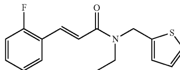
(E)-N-ethyl-3-(2-fluorophenyl)-N-(thiophen-2-ylmethyl)acrylamide
