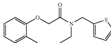
N-ethyl-N-(thiophen-2-ylmethyl)-2-(o-tolyloxy)acetamide
