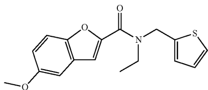
N-ethyl-5-methoxy-N-(thiophen-2-ylmethyl)benzofuran-2-carboxamide
