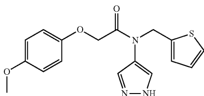
2-(4-methoxyphenoxy)-N-(1H-pyrazol-4-yl)-N-(thiophen-2-ylmethyl)acetamide
