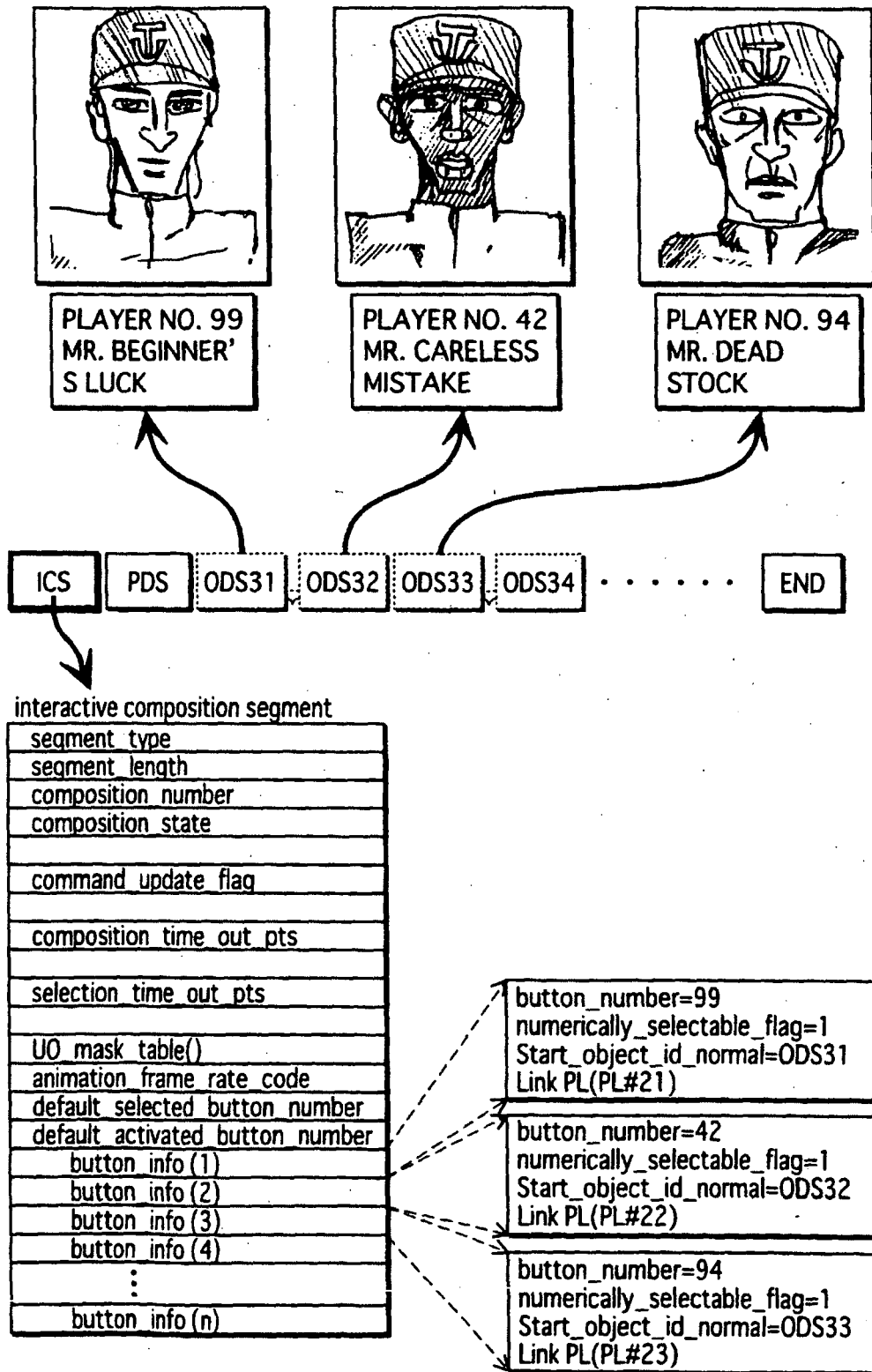
FIG.18 PLAYERS LIST
