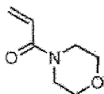
Exemplary Compound 2-6
