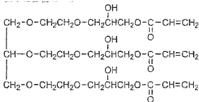
Exemplary Compound 2-3
