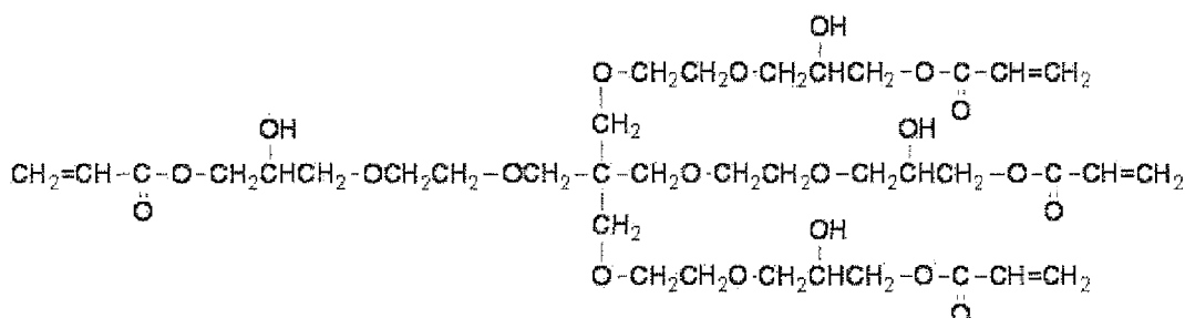
Exemplary Compound 2-2
