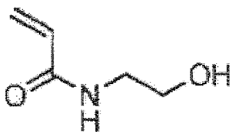
Exemplary compound 2-8
