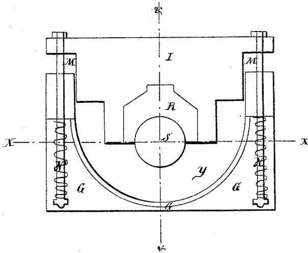
Sectional View
