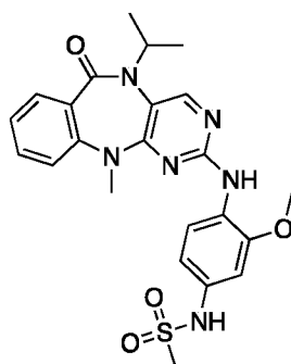
Compound 13: N -(4-((5-isopropyl-11-methyl-6-oxo-6,11-dihydro-5H-benzo[ e ]pyrimido[5,4- b ][1,4]diazepin-2-yl)amino)-3-methoxyphenyl)methanesulfonamide (FMF-03-150-2)
