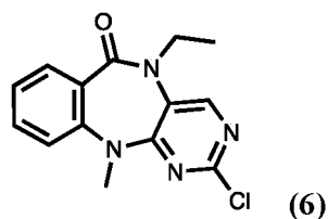
Scheme 3
