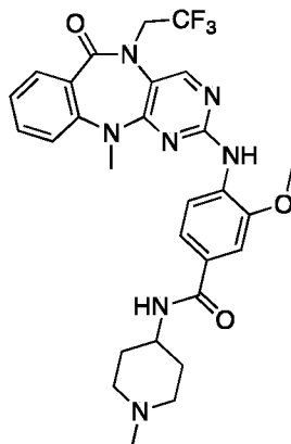
Compound 8: 3-methoxy-4-((11-methyl-6-oxo-5-(2,2,2-trifluoroethyl)-6,11-dihydro-5H-benzo[e]pyrimido[5,4-b][1,4]diazepin-2-yl)amino)-N-(1-
