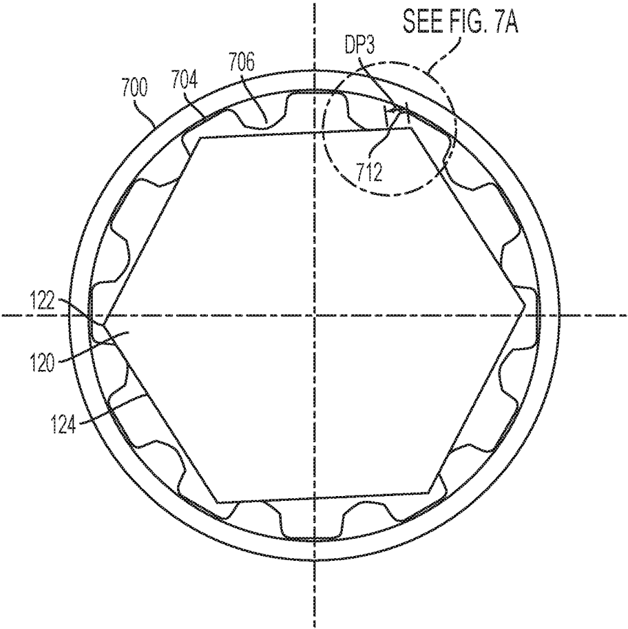
FIG. 7 PRIOR ART
