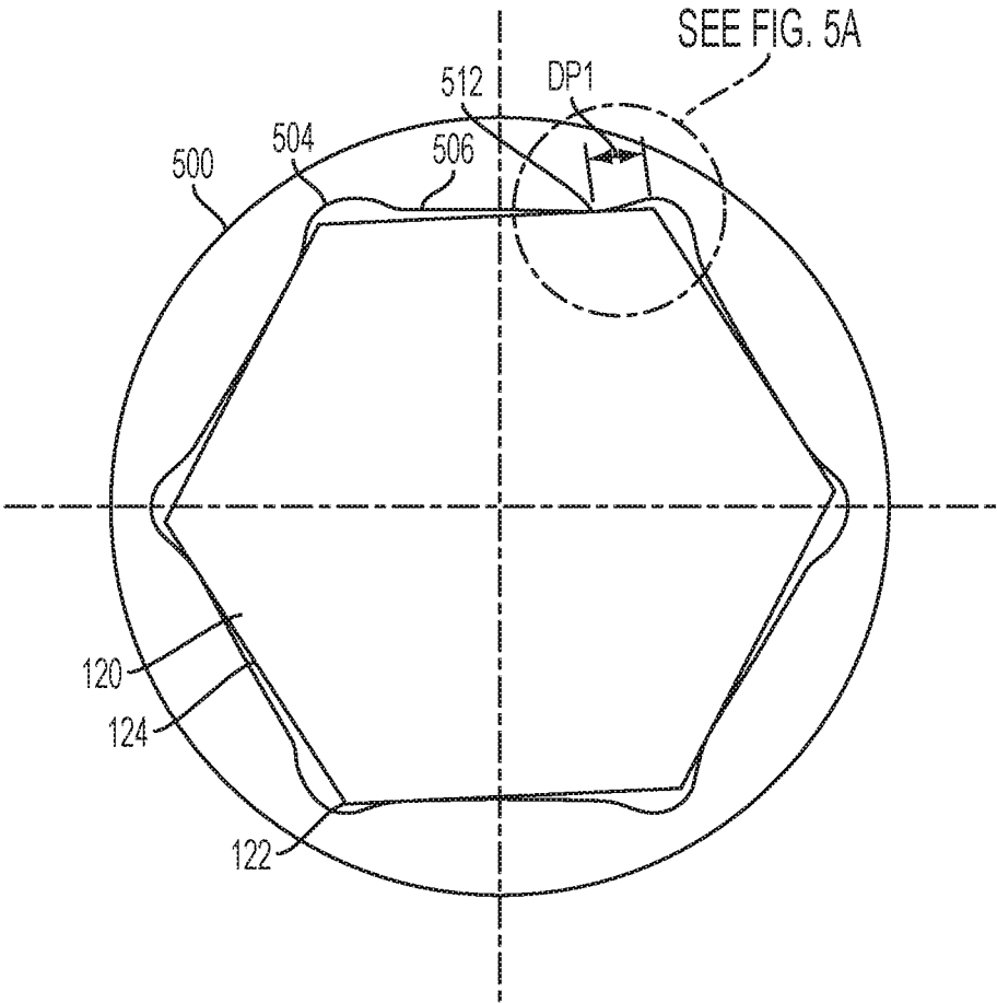
FIG. 5 PRIOR ART
