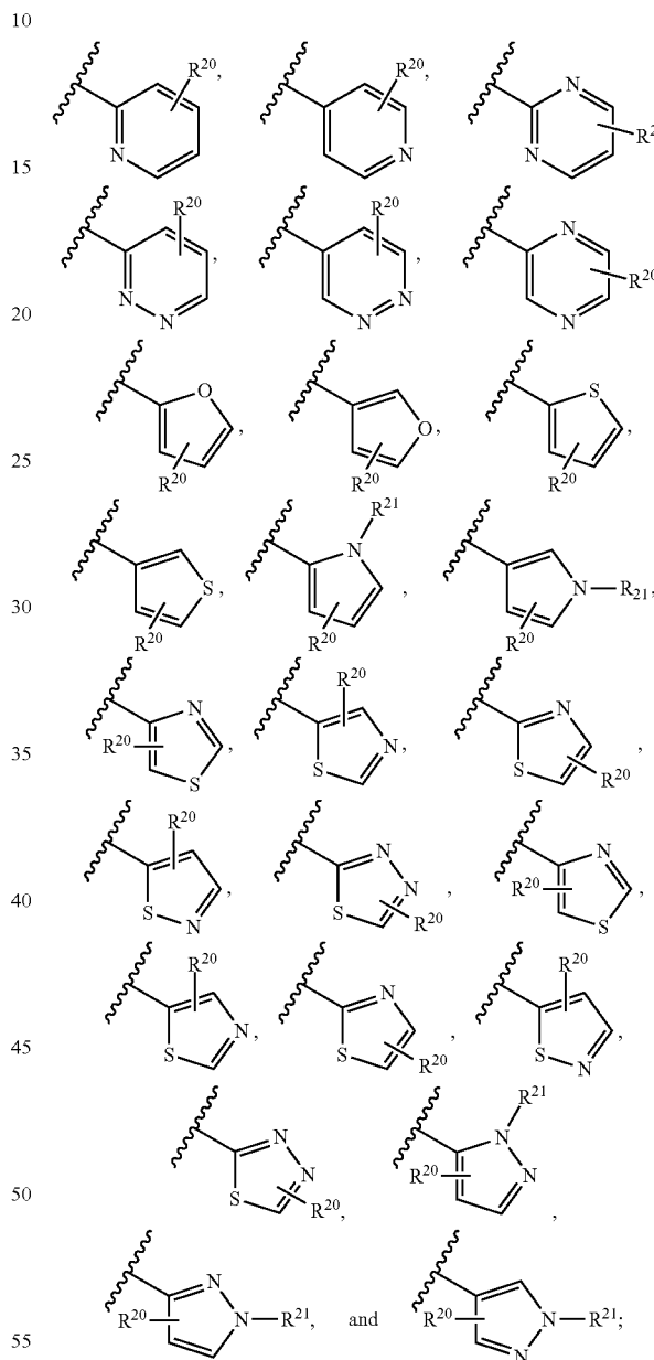
(Formula IVd)
