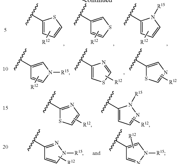
(Formula 1e)
