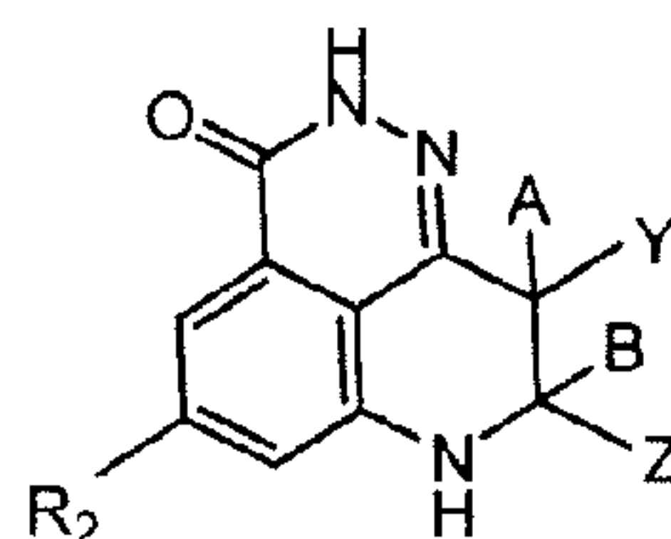
Formula (II);
