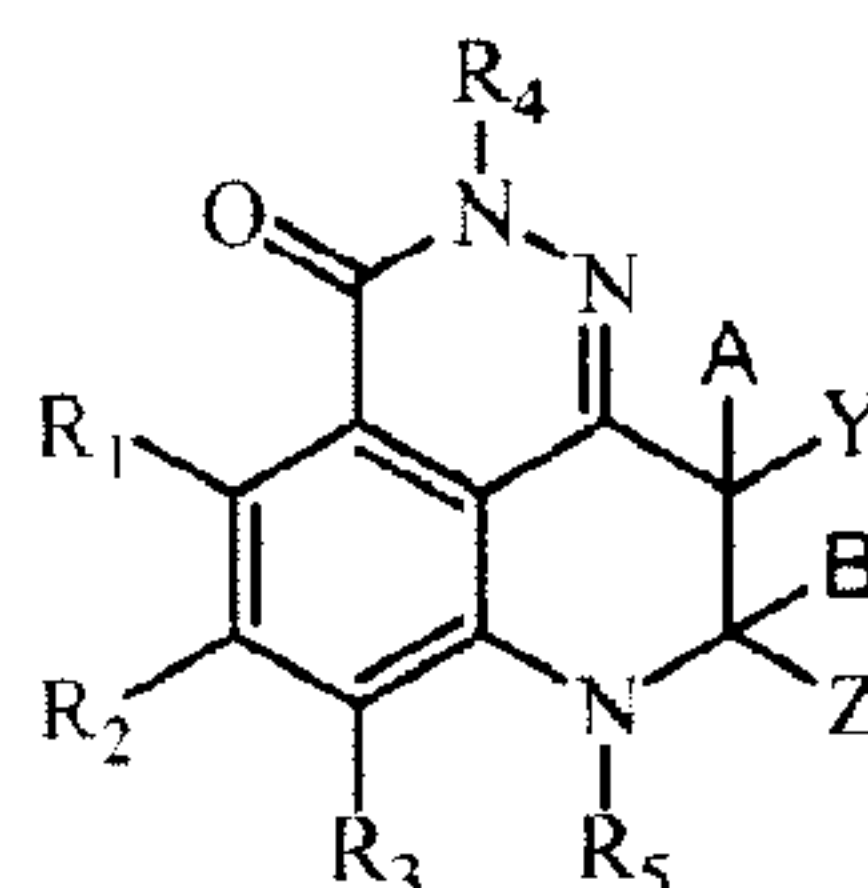
Formula (I)
