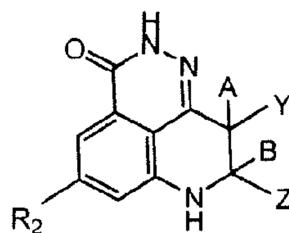
Formula (II);
