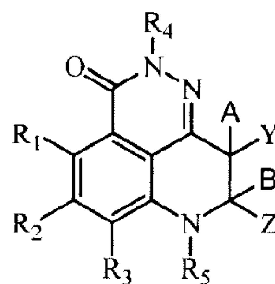
Formula (I)
