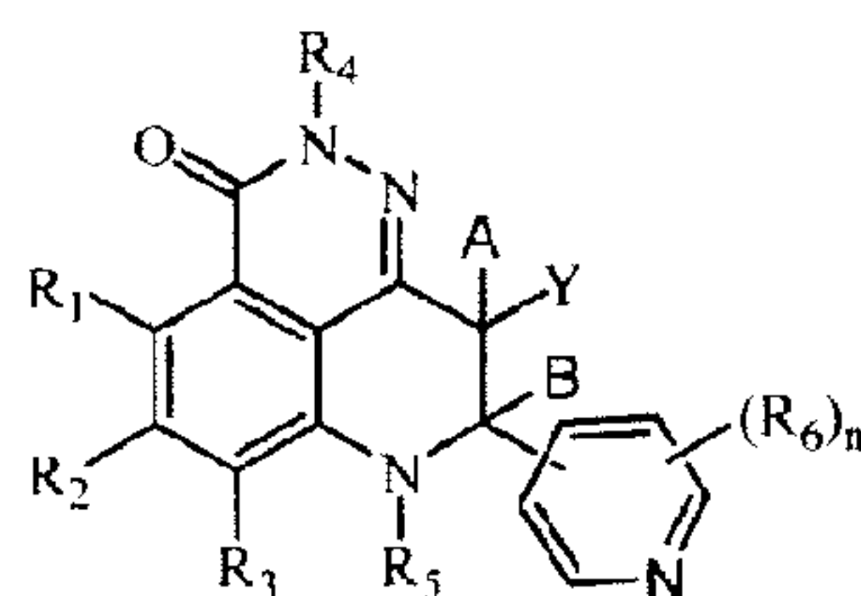
Formula (IA)
