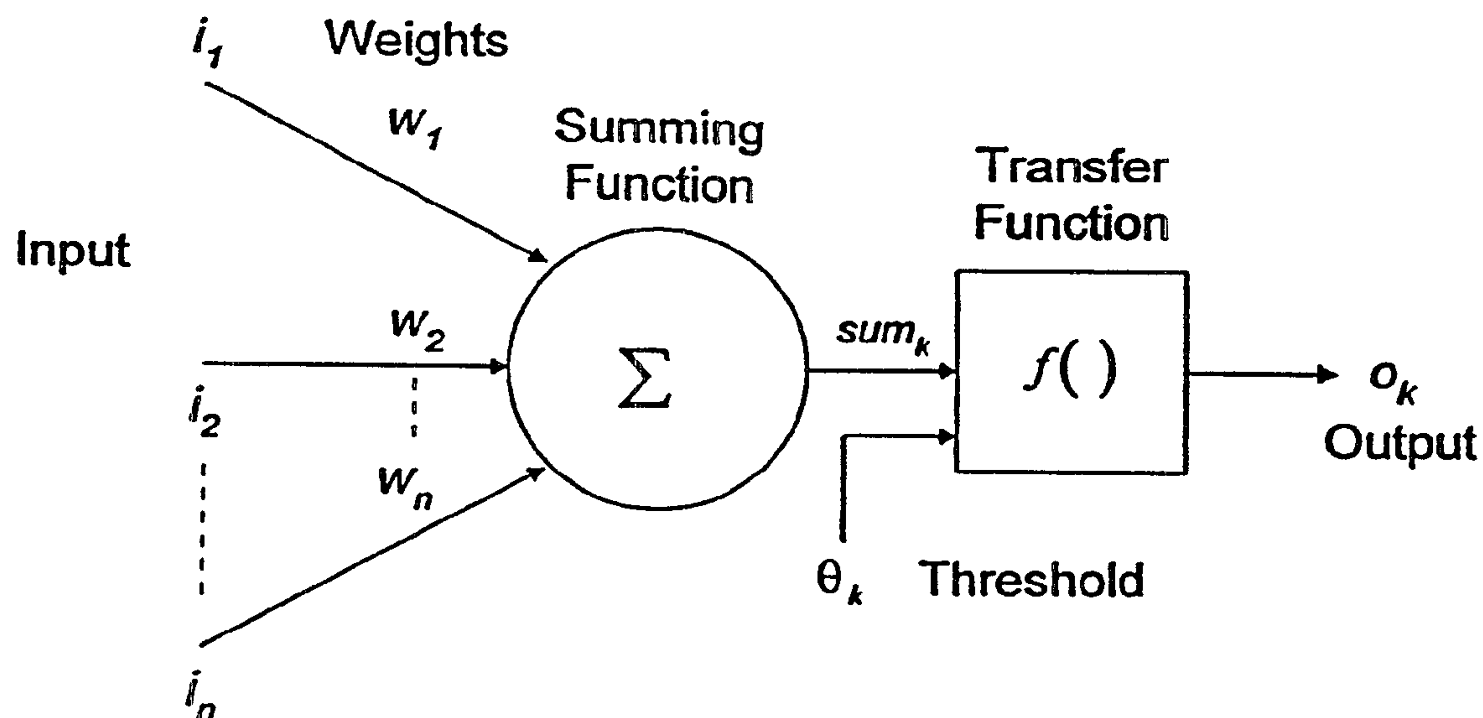
Neuron Diagram
