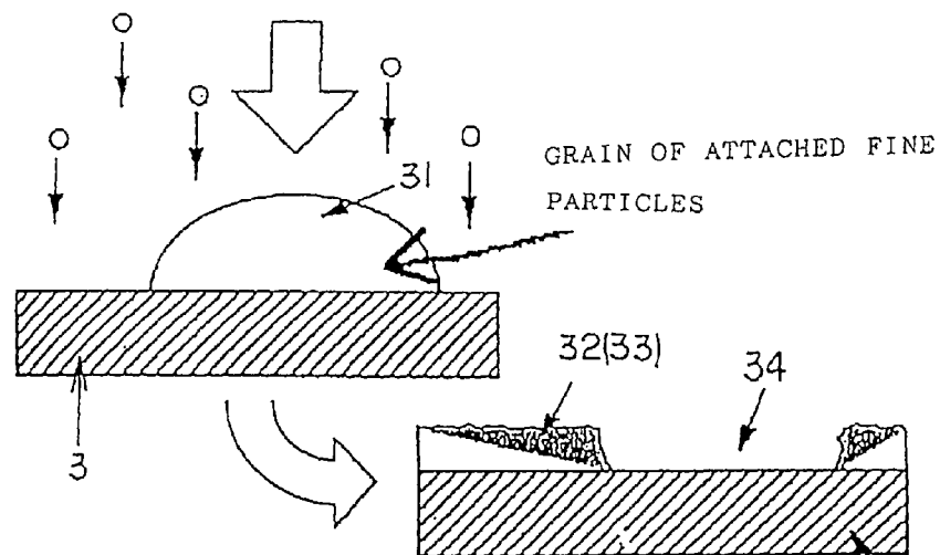
(a) OBSTRUCTION OF ATTACHED FINE PARTICLES AGAINST NORMAL DEPOSITION
