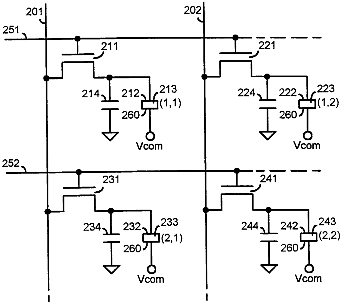
fig.2 prior art
