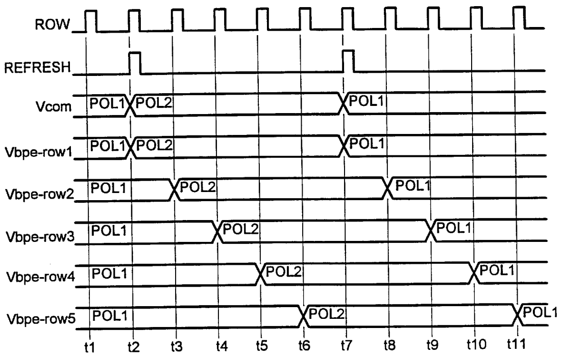
fig.4 prior art
