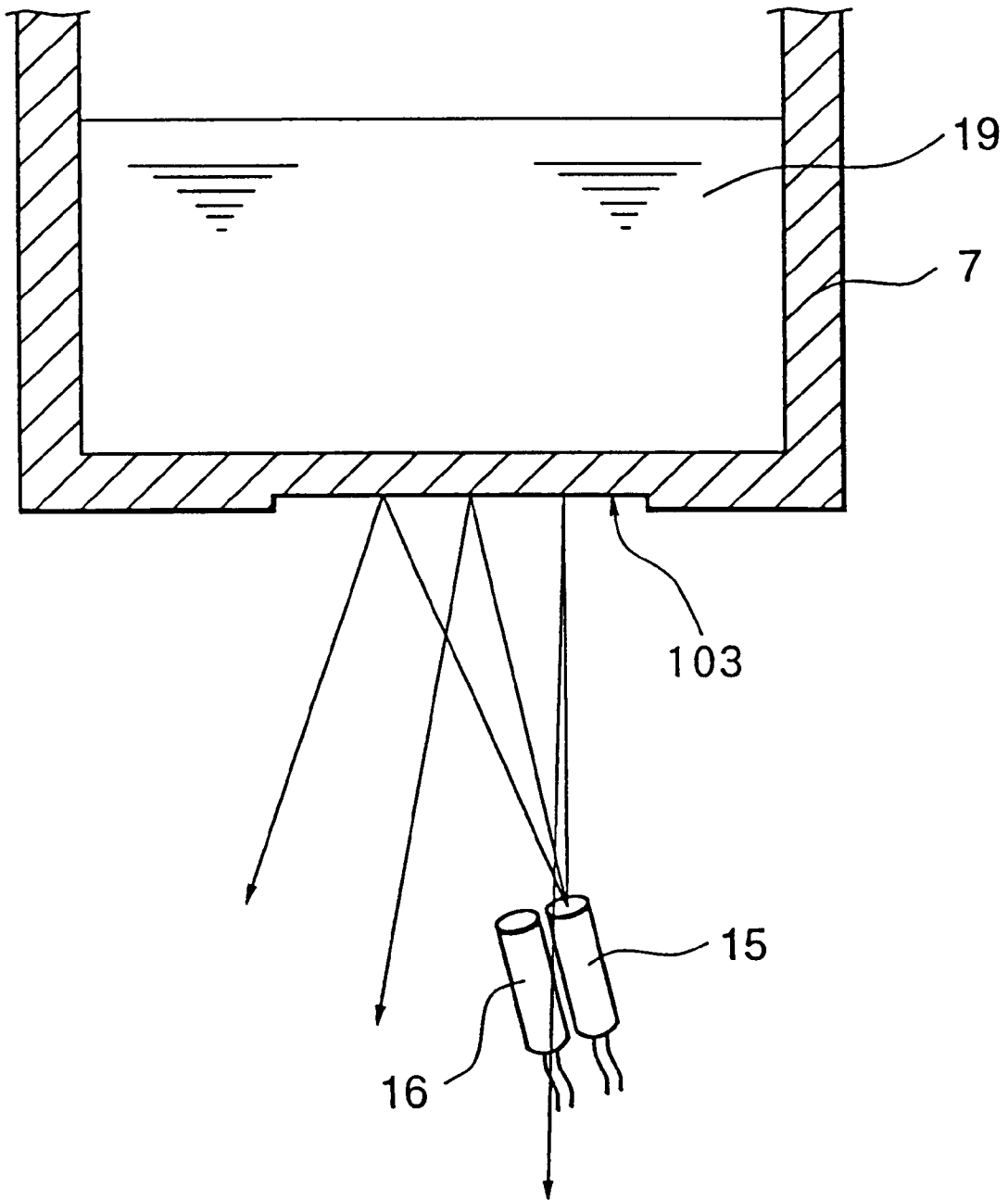
FIG. 10C PRIOR ART
