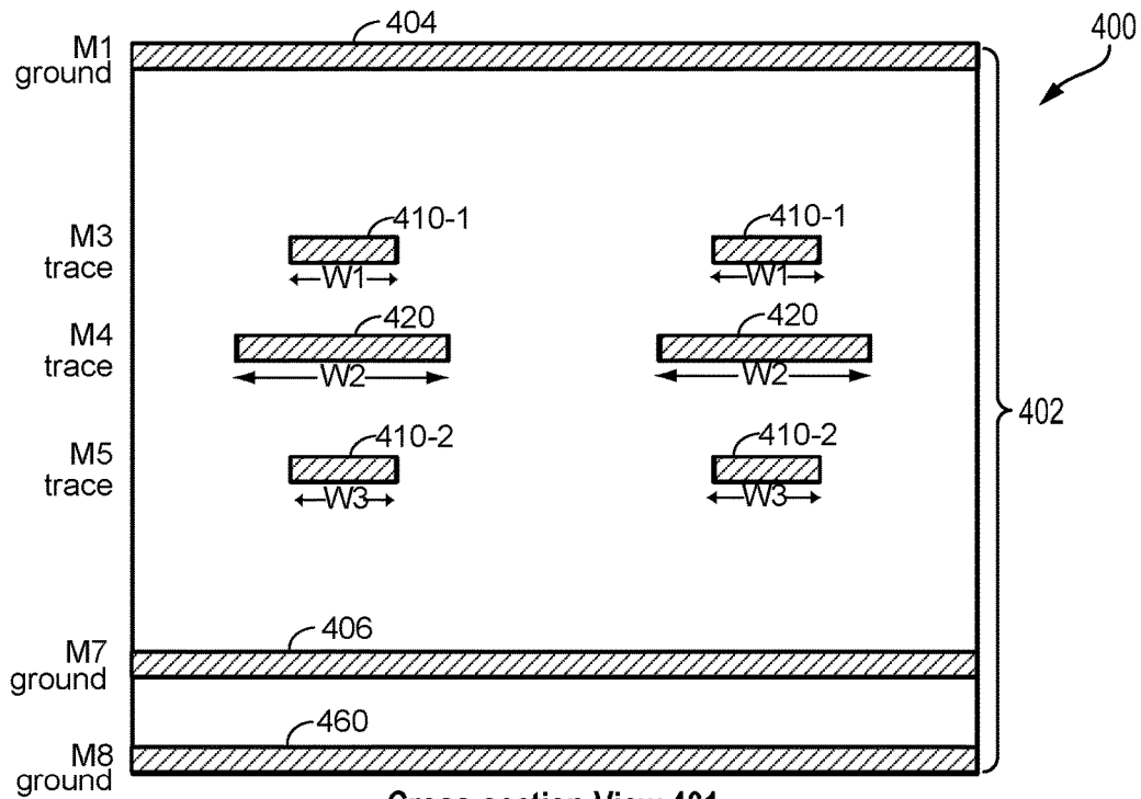
Cross-section View 401
