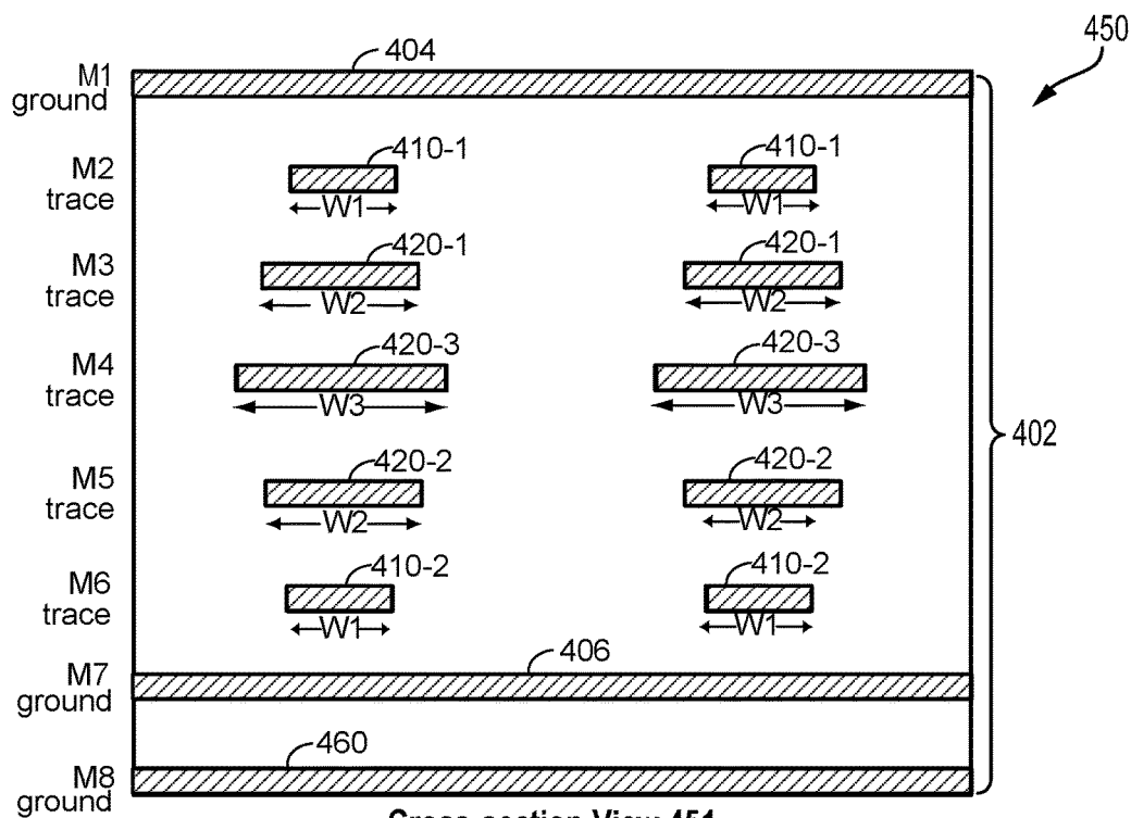
Cross-section View 451
