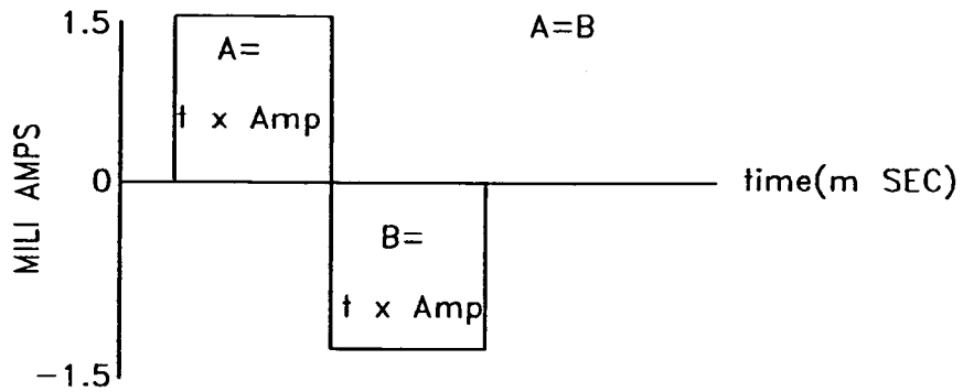
BALANCED BIPHASE WAVE FOR
