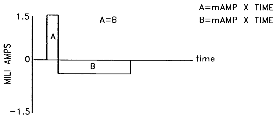
ASYMMETRIC WAVE FORM ENHANCED ANODAL BLOCK
