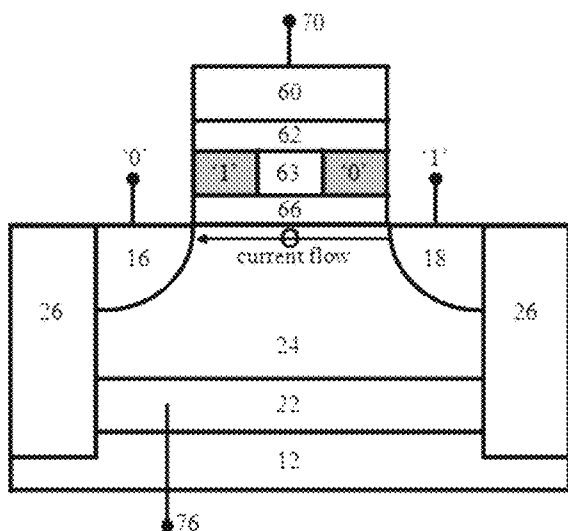
Data bit '1' Search bit '0'
