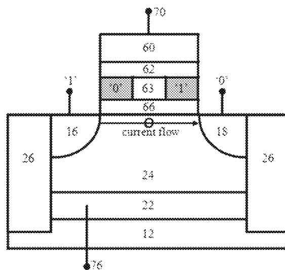
Data bit '0' Search bit '1'
