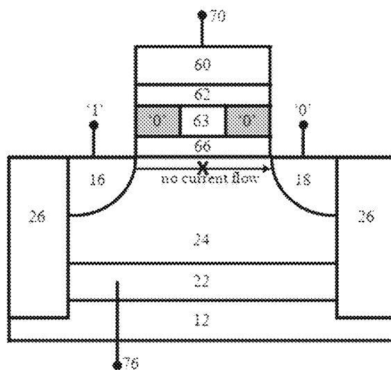
Data bit 'X' Search bit '1'
