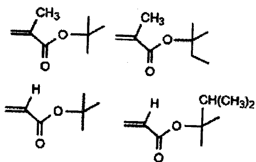
[Chem. 48]
