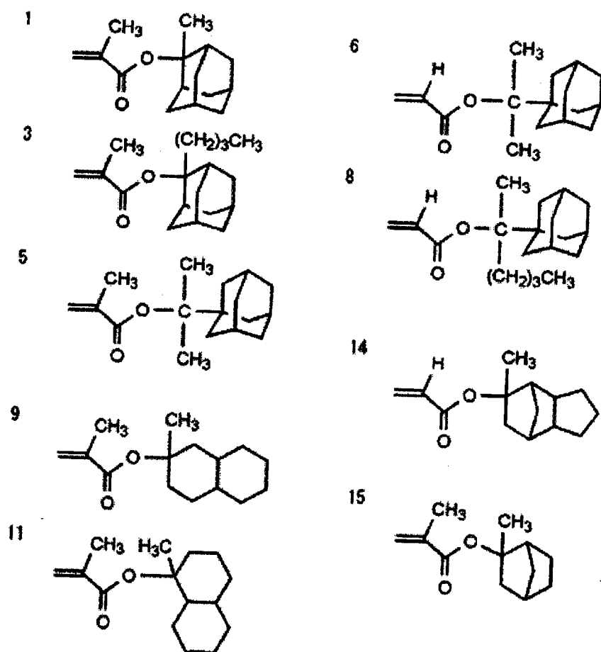
[Chem. 49]
