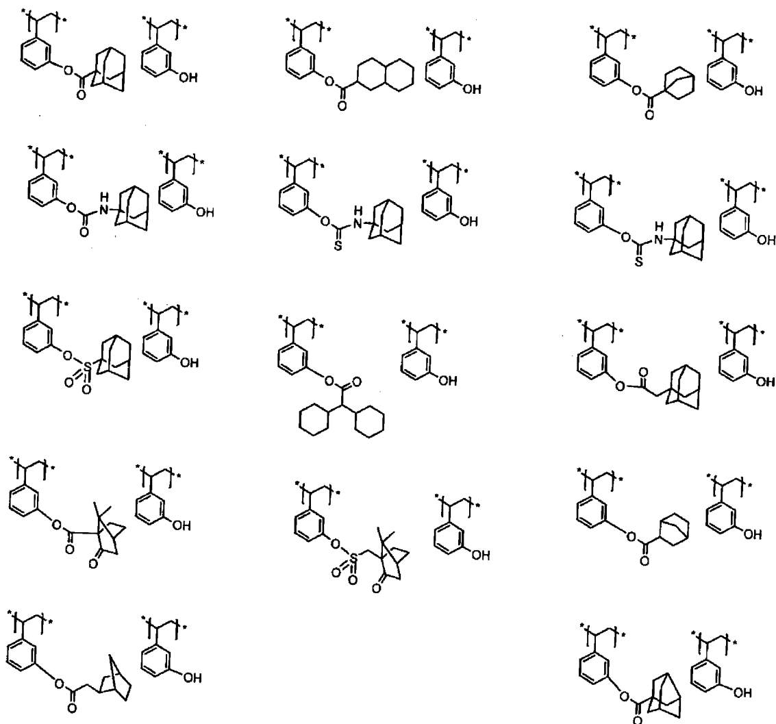
[Chem. 33]
