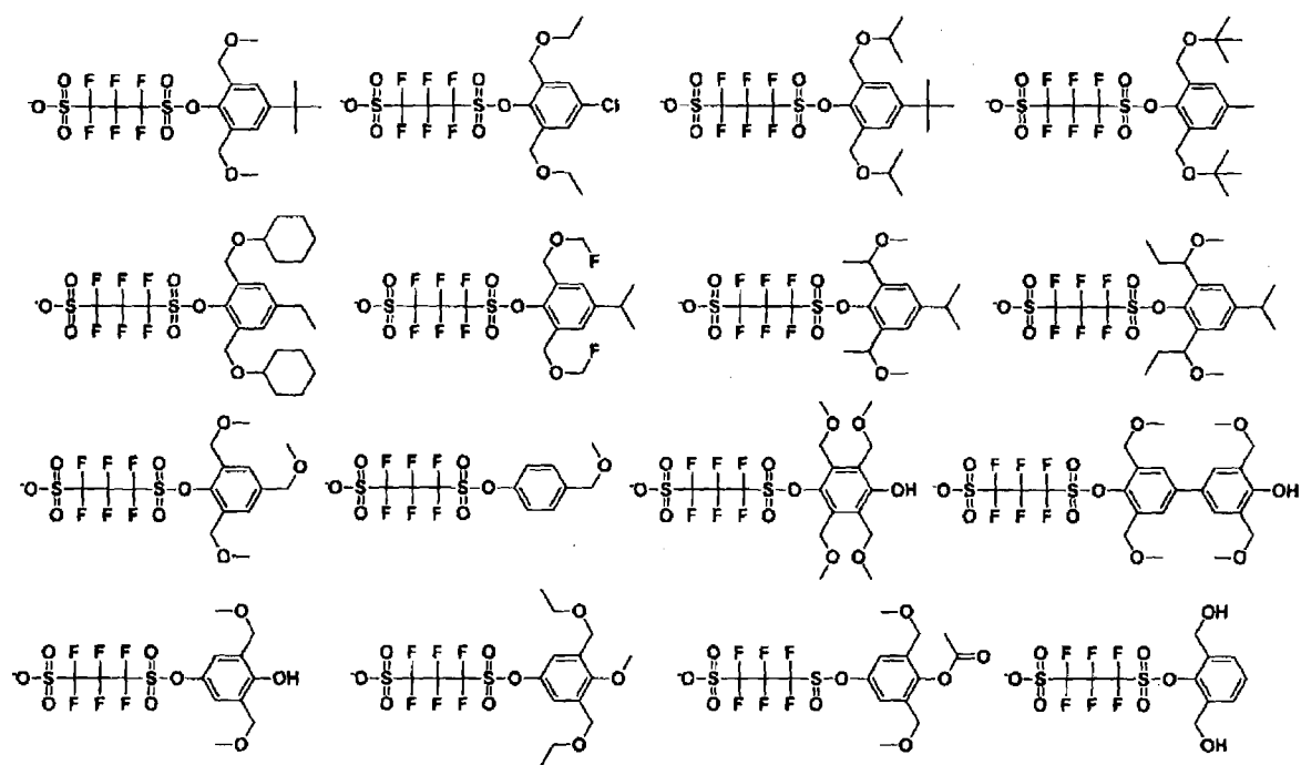
[Chem. 17]
