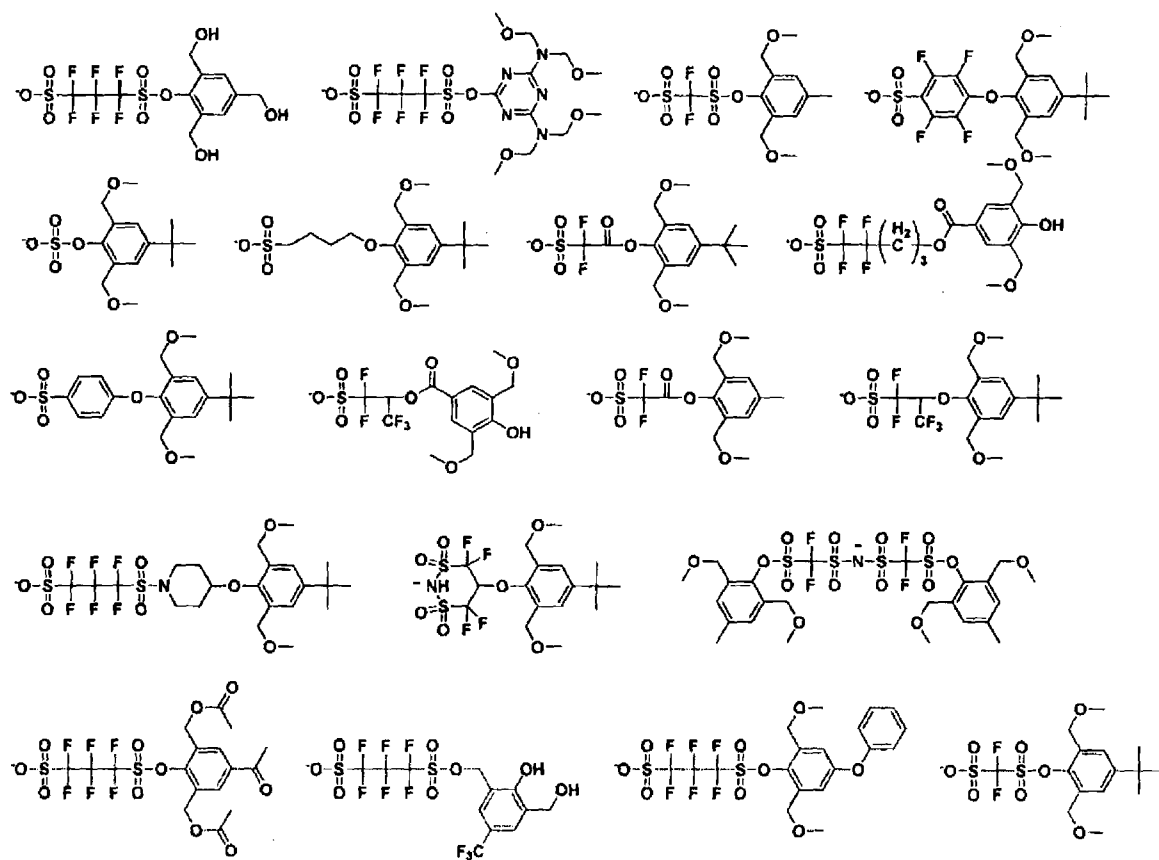
[Chem. 18]
