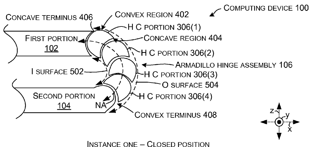
INSTANCE ONE – CLOSED POSITION
