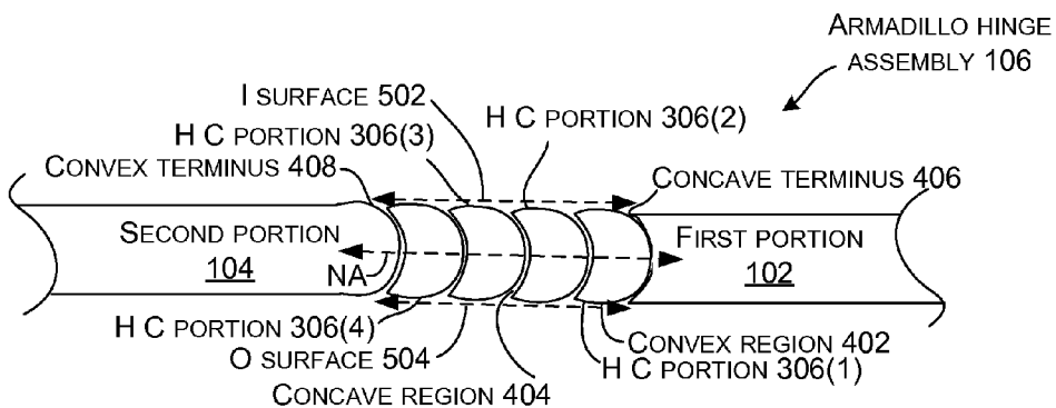
INSTANCE THREE – FULL-OPEN POSITION
