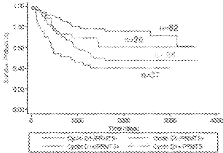
Survival Estimates - Cyclin D1 Stain Proportion Status*PRMT5 Nuclear Stain Intensity Status Interaction
