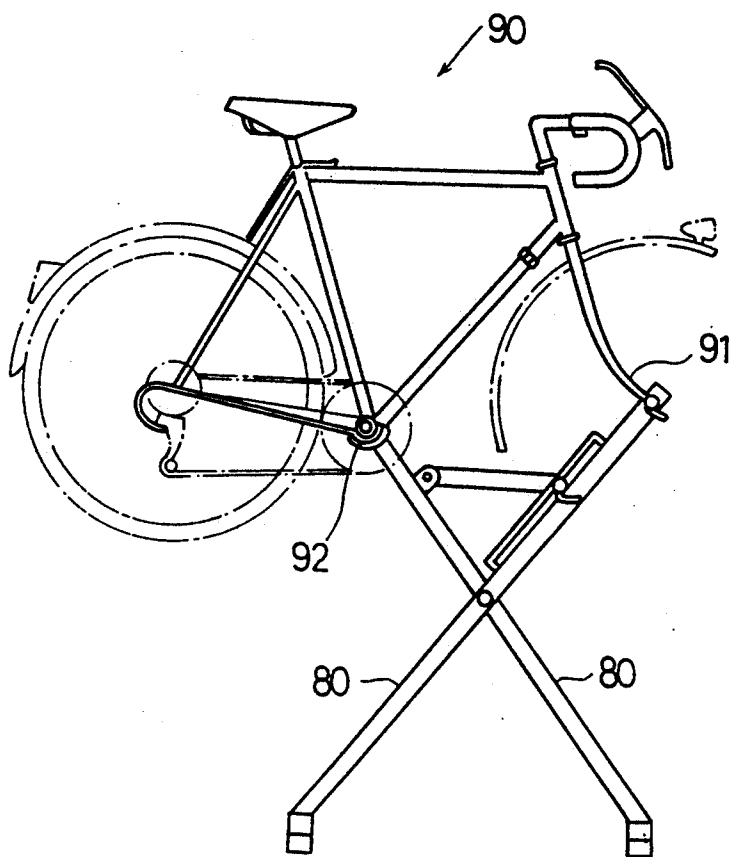
Fig. 12(Prior Art)
